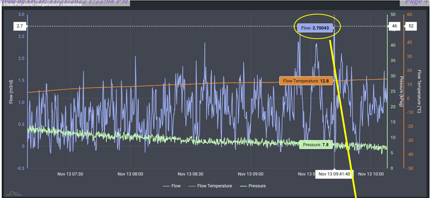
Image 4.1 – Fowler Hair #001 (30-025-11103) Methane Flow/Pressure/Temperature Timeseries & Peak Flow at Interval #1 testing period of 3.0-hours.
