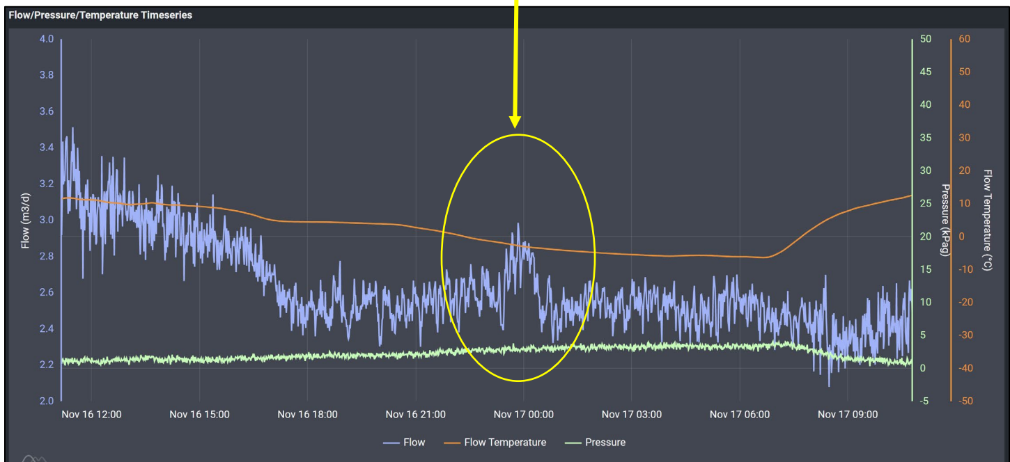
Image 4.2 – Double L Queen #01Y (30-005-60084) Methane Flow/Pressure/Temperature Timeseries &amp; Peak Flow for entire testing period or 23.6-hours.
