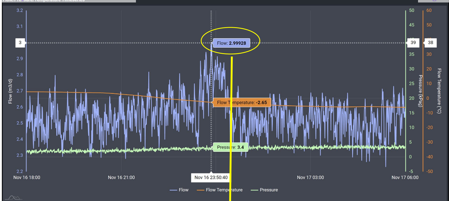
Image 4.1 – Double L Queen #01Y (30-005-60084) Methane Flow/Pressure/Temperature Timeseries &amp; Peak Flow at Interval #1 testing period of 12.0-hours.
