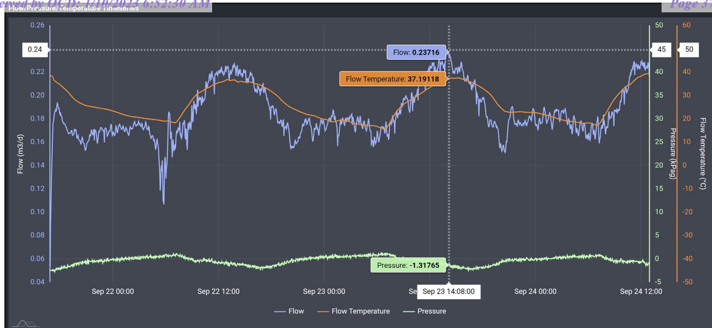
Image 4.1 – Double L Queen #01Q (30-005-20327) Methane Flow/Pressure/Temperature Timeseries &amp; Peak Flow
