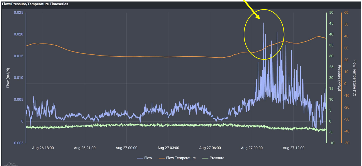
Image 4.2 – TLSA #005 (30-005-60572) Methane Flow/Pressure/Temperature Timeseries & Peak Flow for entire testing period of 21.6-hours.
