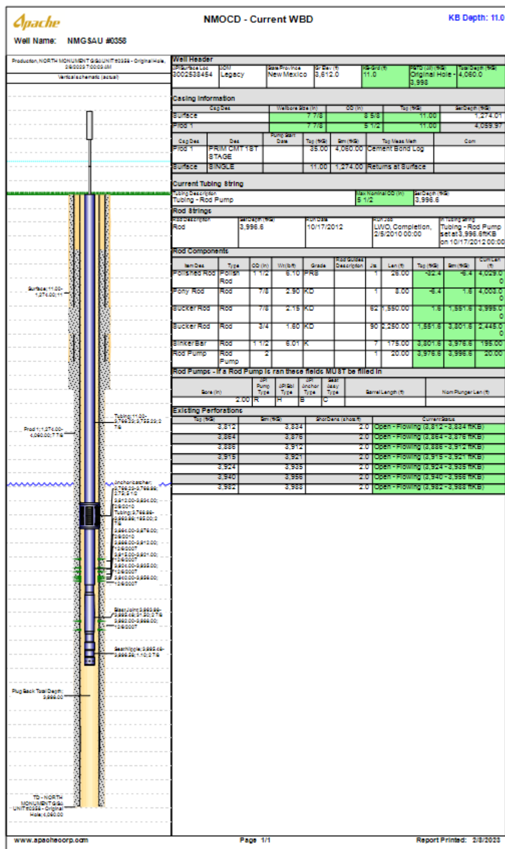
Figure 1 – Current Wellbore Diagram
