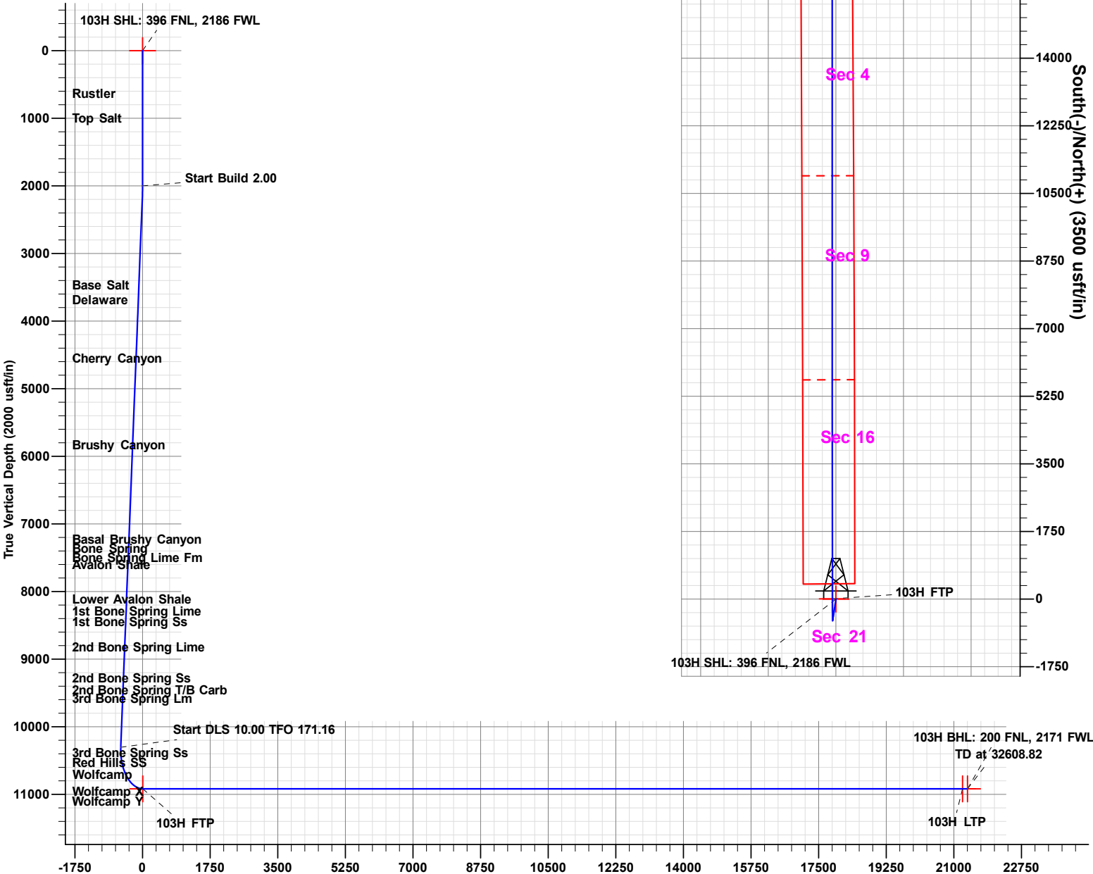
Vertical Section at 359.98° (3500 usft/in)
