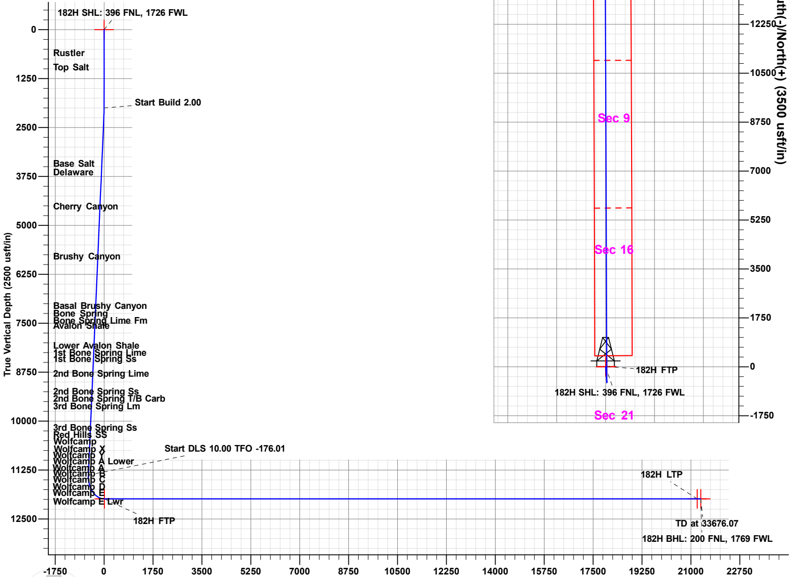
Vertical Section at 359.77° (3500 usft/in)
