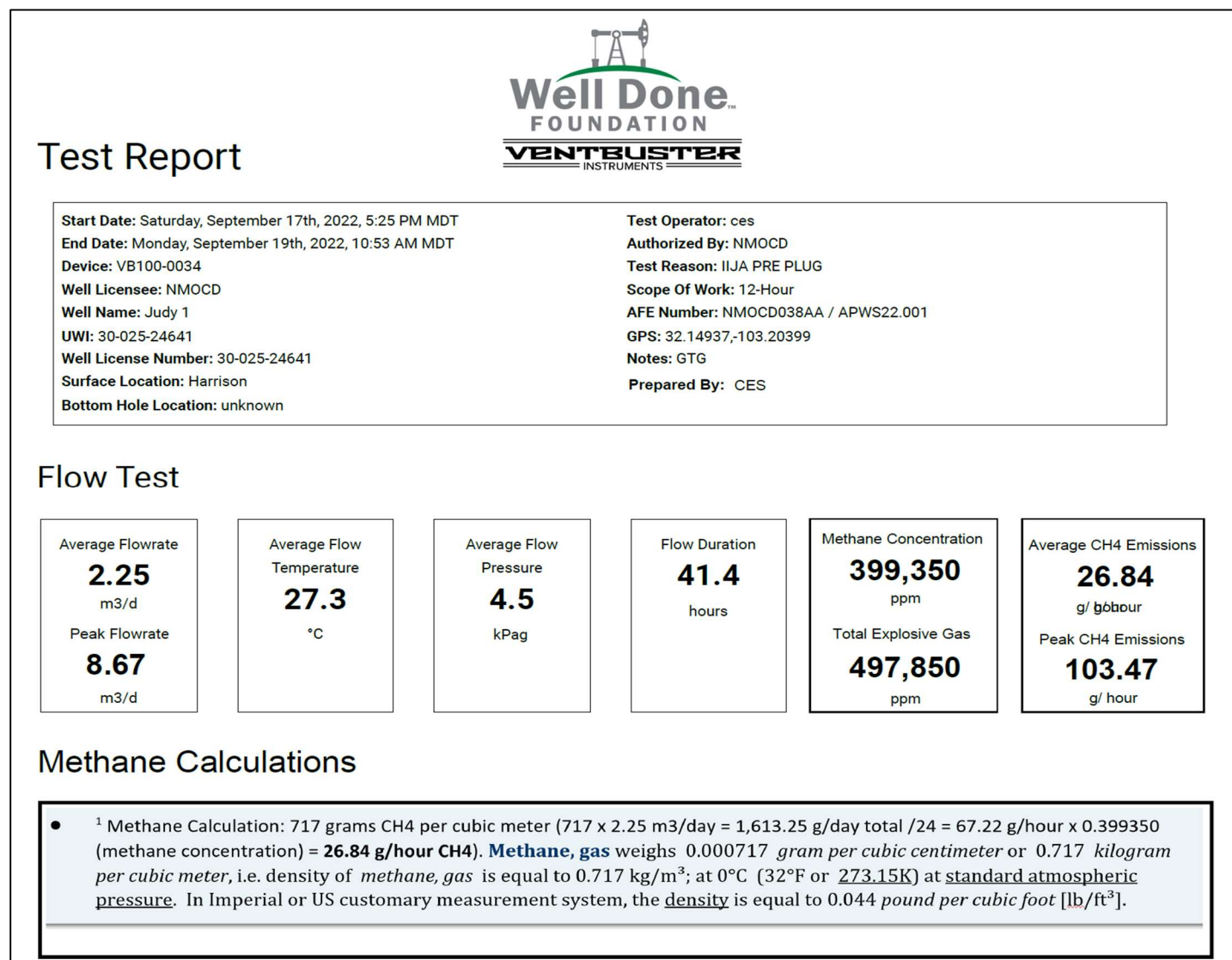
Image 2.1 – Judy #001 (30-025-24641) Methane Monitoring Dashboard
