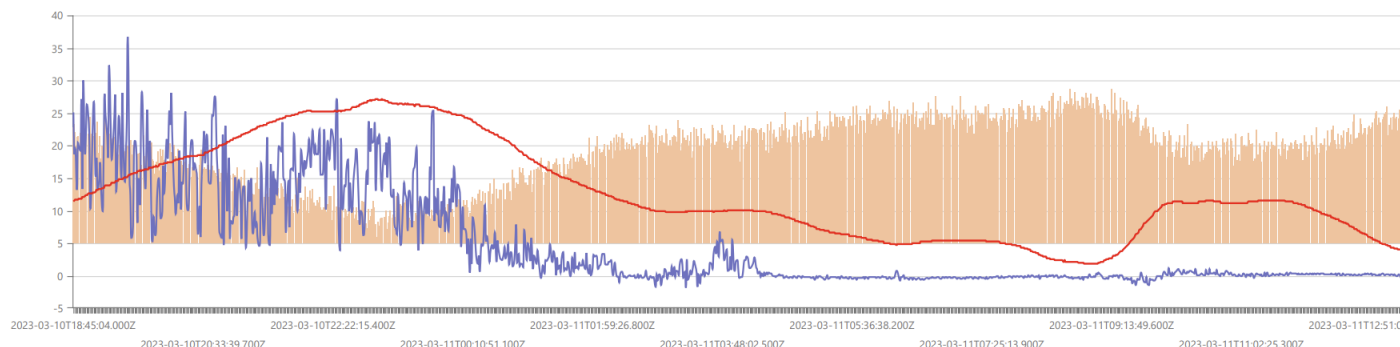
Image 2.1 – Artesia Metex #038 Pre Plugging Test Report
