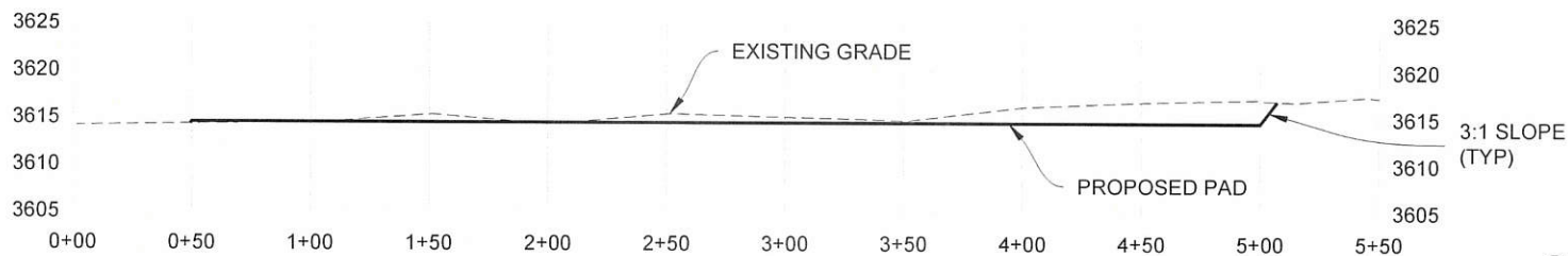
SECTION C-C'
