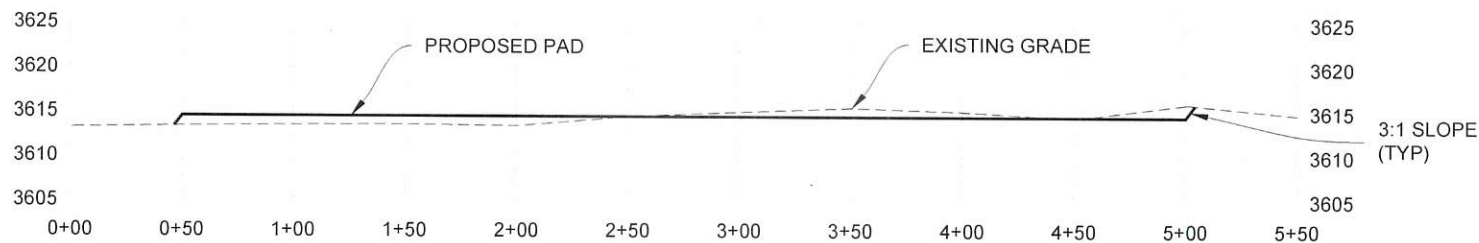
SECTION B-B'
