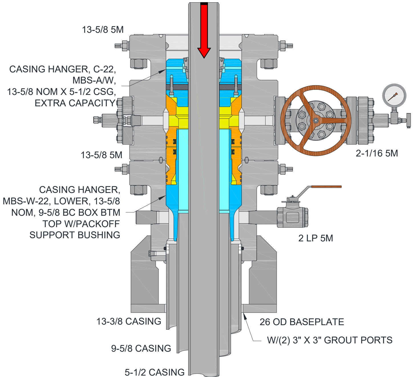
FIGURE 4 – HANGER INSTALLED
