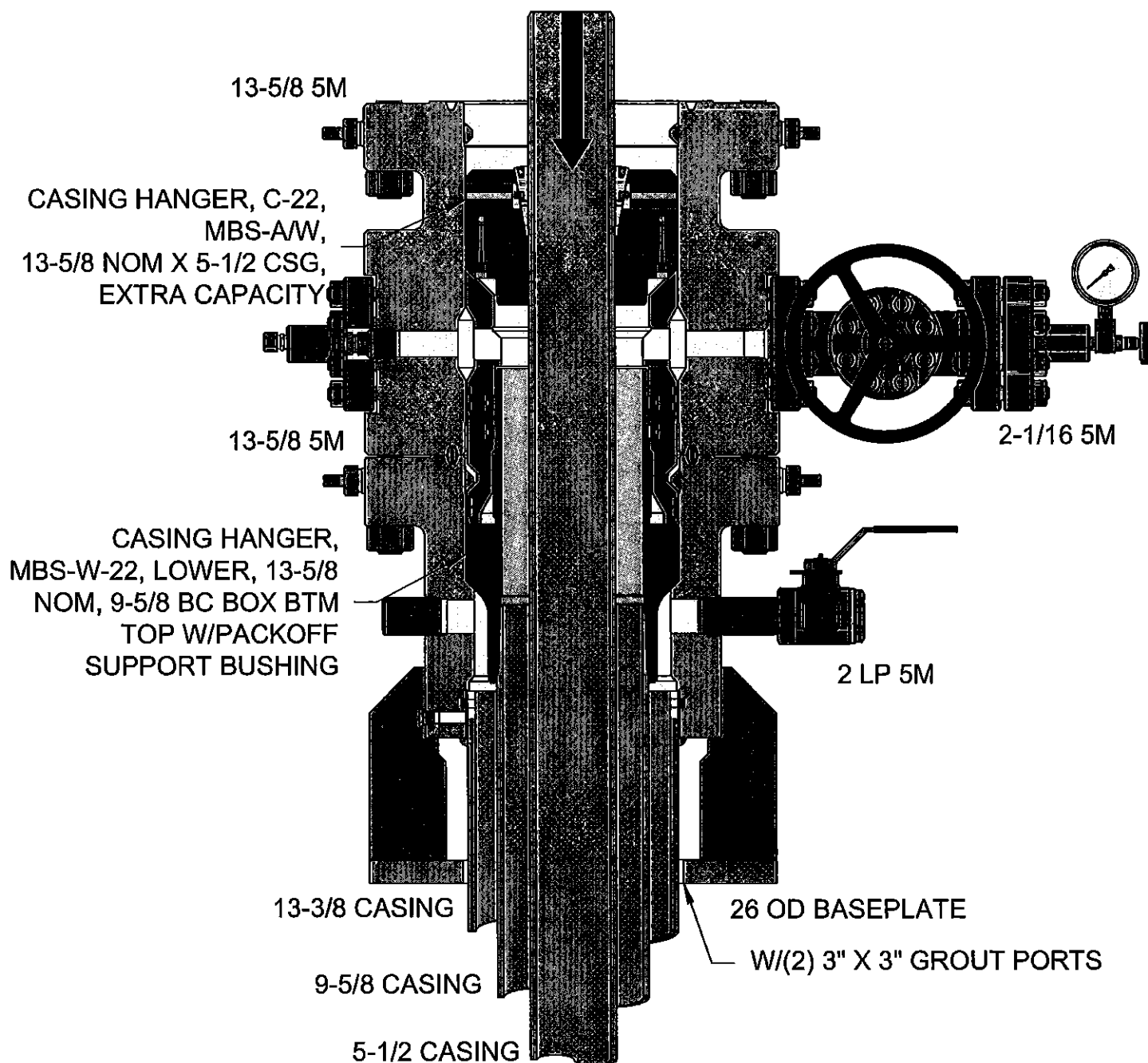
FIGURE 4 – HANGER INSTALLED
