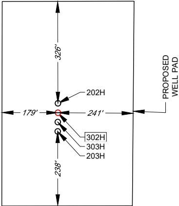
DETAIL VIEW SCALE: 1" = 300'
