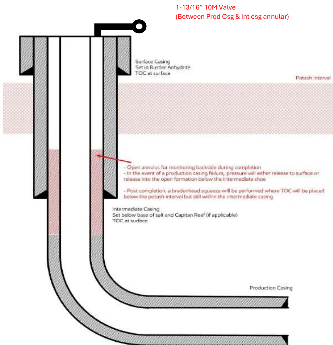
Figure B – 3 String design
