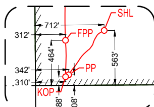
DETAIL VIEW SCALE: 1" = 1000'
