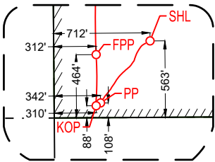
DETAIL VIEW SCALE: 1" = 1000'
