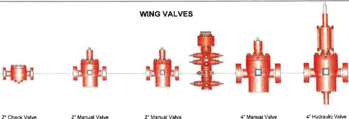
2" Check Valve
