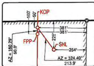
DETAIL VIEW SCALE: 1" = 400'
