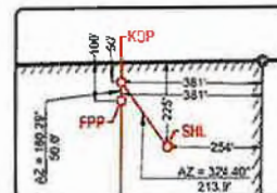
DETAIL VIEW SCALE: 1" = 400'
