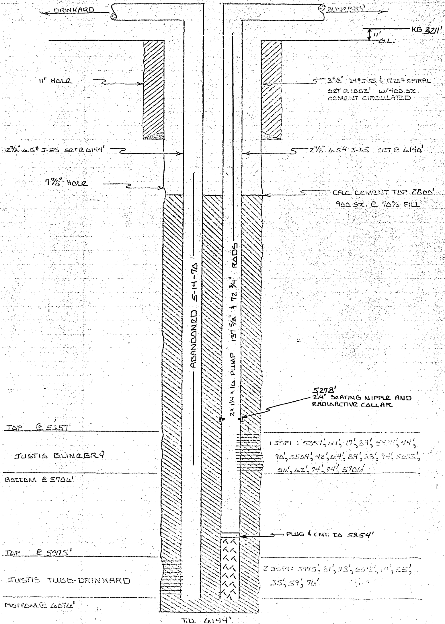
C.C. FRISTAL "B" FLD. (NCT-1) N° 2 SUBJECT WELL PRESENT WELLBORE DIAGRAM
