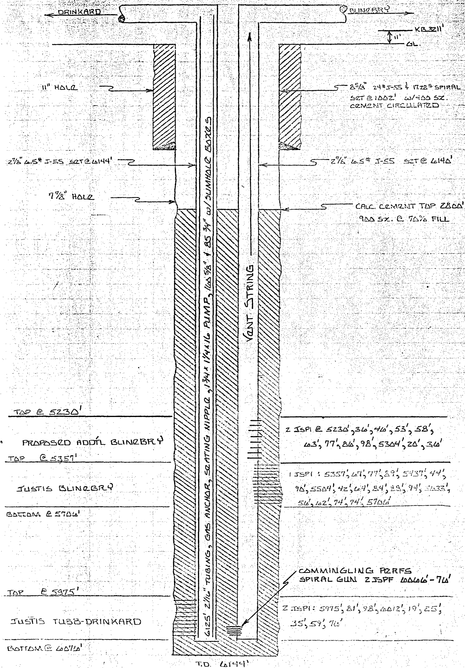
C.C. FRISTOL "B" F.R.D. (NCT-1) No 2 SUBJECT WELL PROPOSED WELLBORE DIAGRAM
