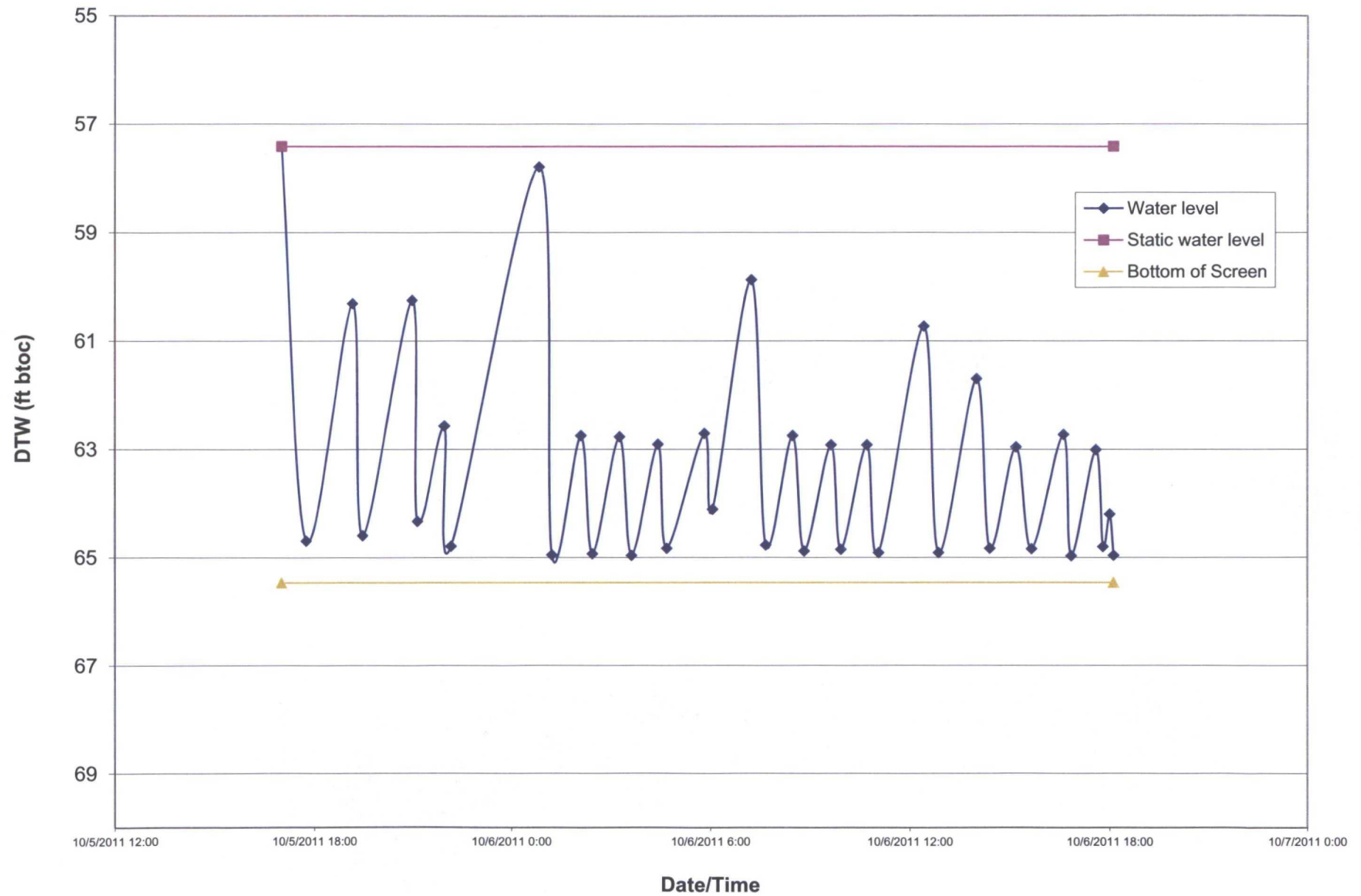
Depth to Water During Bail Down Test of Well 5-16B
