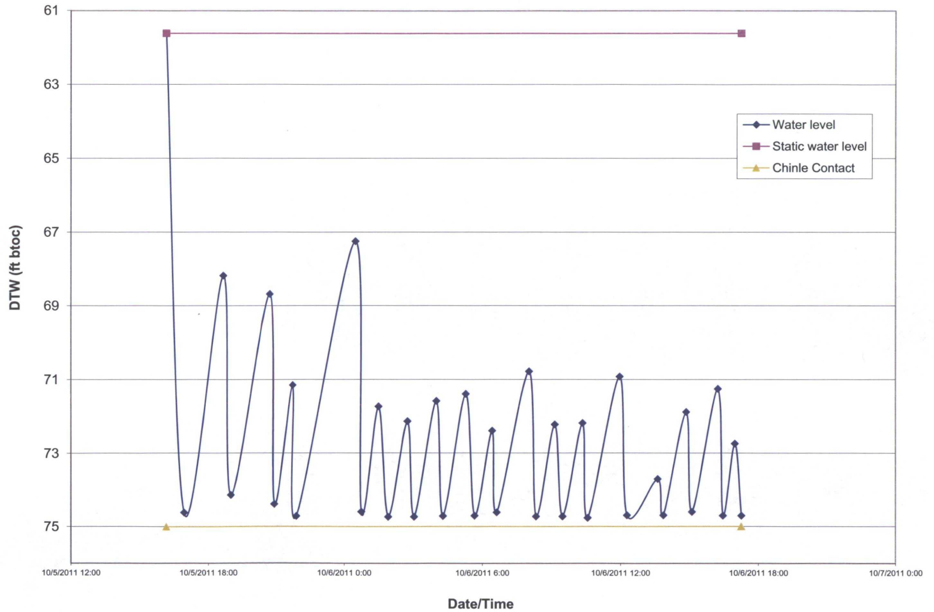
Depth to Water During Bail Down Test of Well 5-24B
