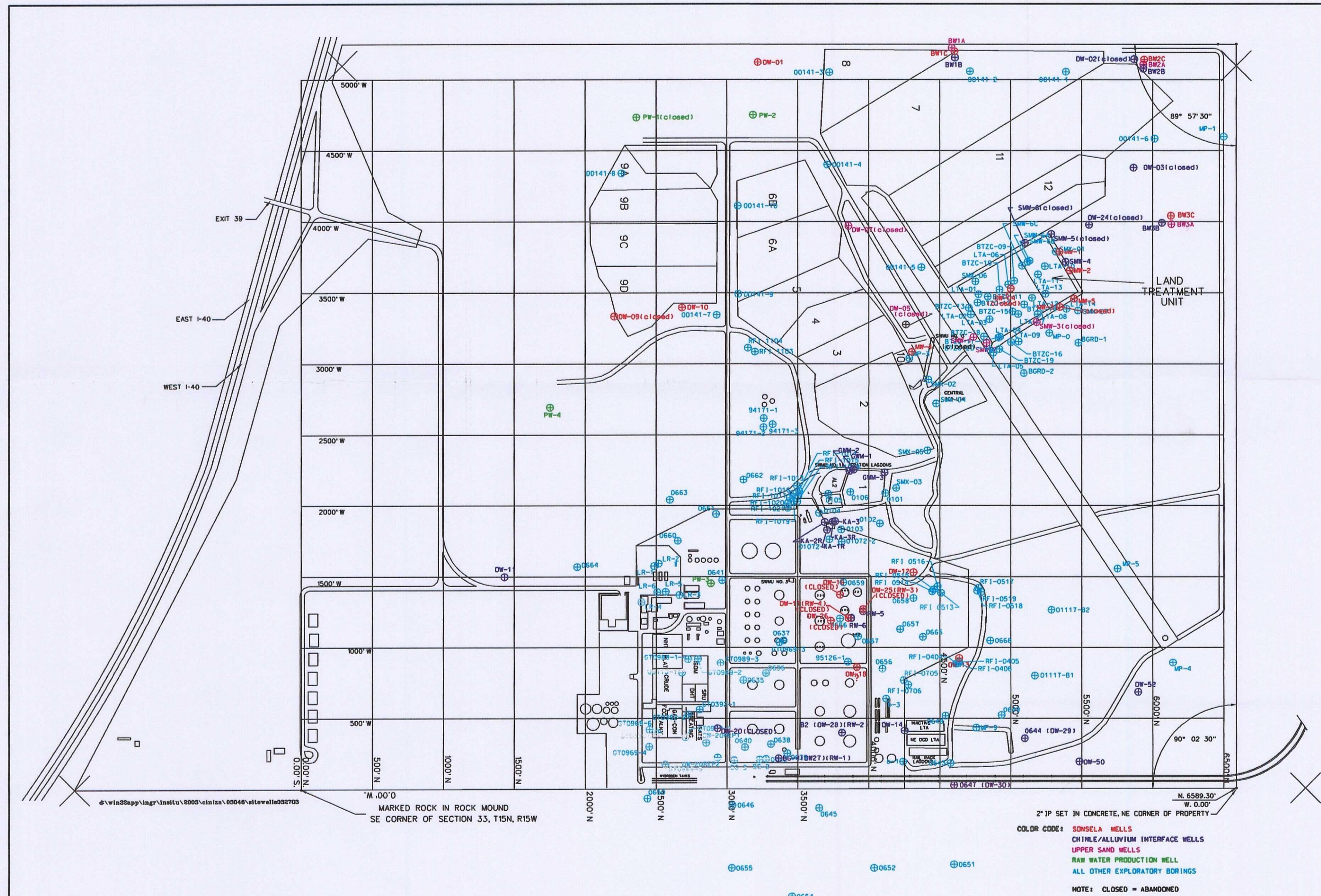
Figure 7 Well and Boring Locations Map (Historic/Current) As of December 2009 Western Refining - Gallup Refinery Interstate 40, Exit 39 Jamestown, New Mexico 87347 Date: August 23, 2010
