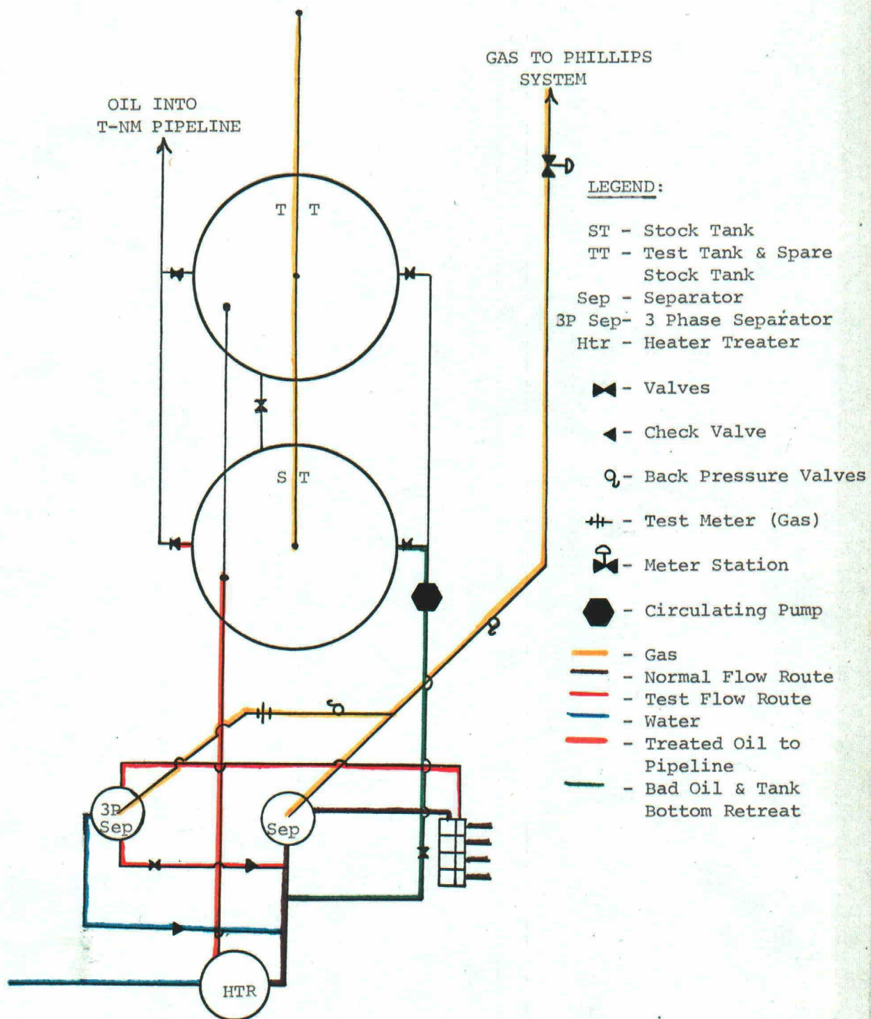
GETTY OIL COMPANY SCHEMATIC DIAGRAM OF PROPOSED COMMINGLING FACILITIES STATE "D" AND STATE "E" LEASES EUNICE-MONUMENT GRAYBURG SAN ANDRES LEA COUNTY, NEW MEXICO
