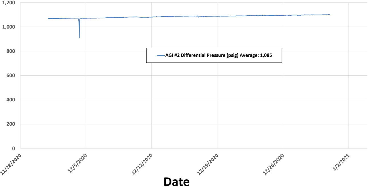
FIGURE #7: LINAM AGI #2 TAG INJECTION PRESSURE AND CASING ANNULAR PRESSURE DIFFERENTIAL (PSIG)
