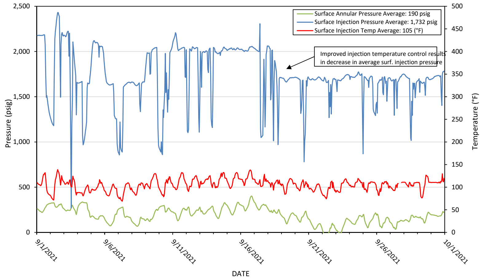
FIGURE 3. INDEPENDENCE AGI #1 SURFACE INJECTION PRESSURE, ANNULAR PRESSURE AND INJECTION TEMPERATURE
