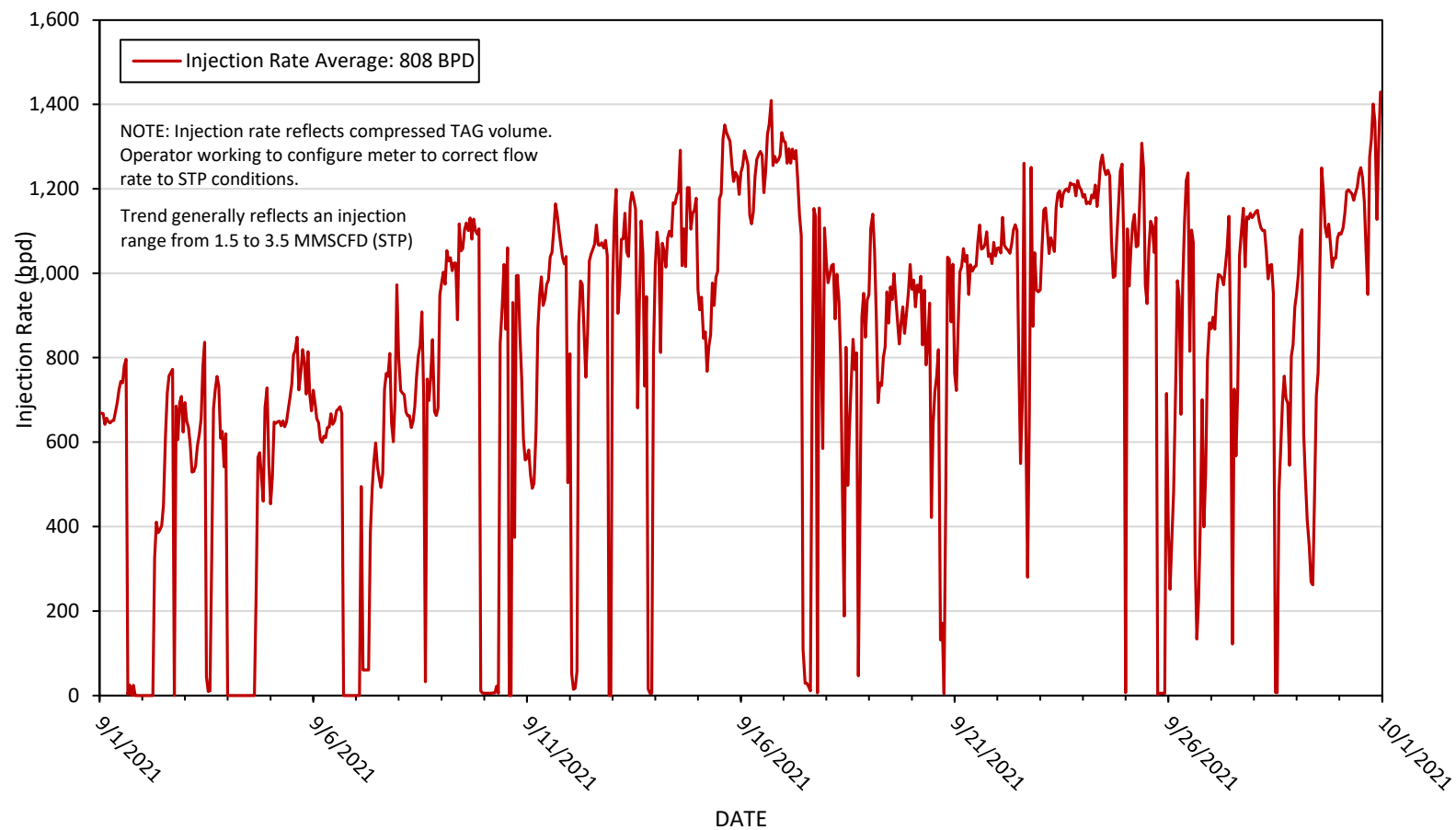
FIGURE 1 - INDEPENDENCE AGI #1 INJECTION RATES WHILE OPERATING
