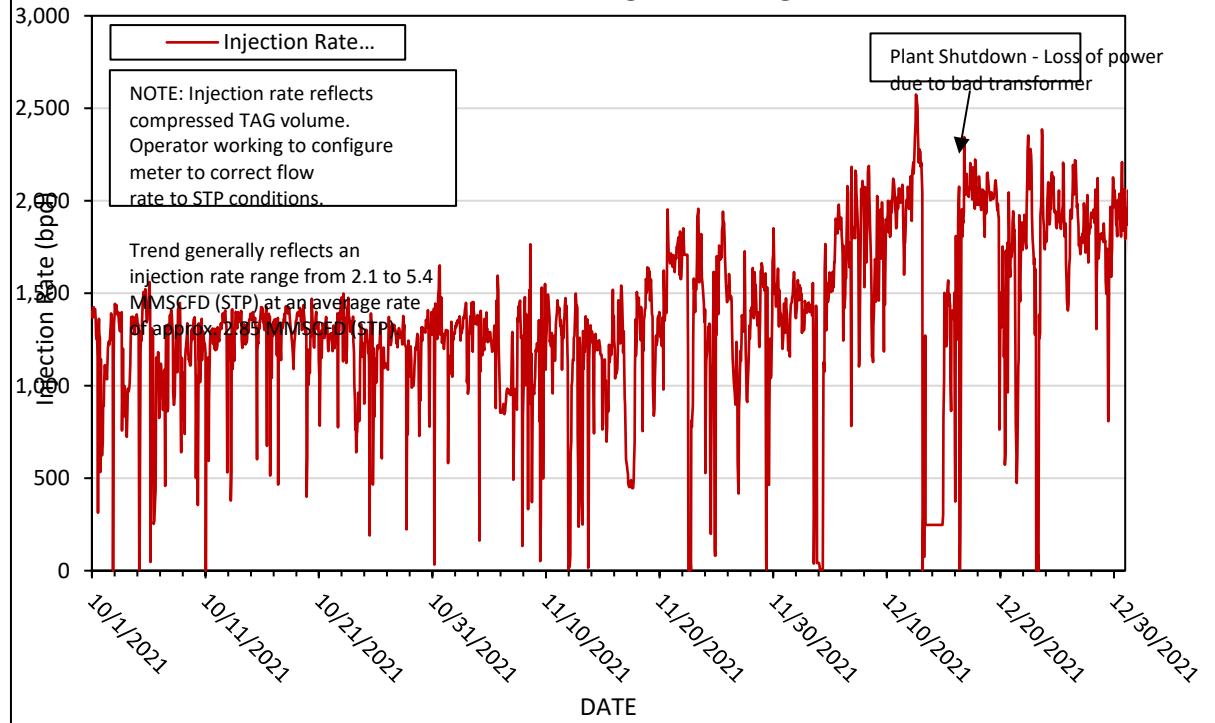
FIGURE 1 - INDEPENDENCE AGI #1 INJECTION RATES WHILE OPERATING
