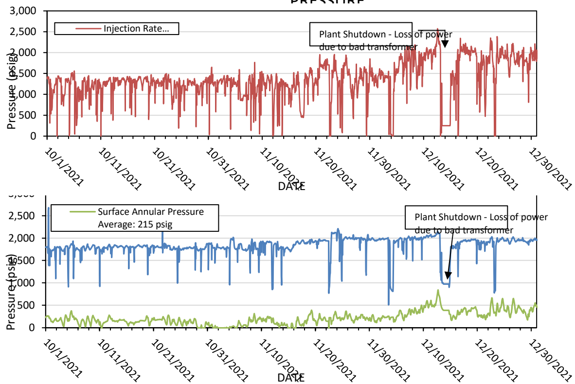
FIGURE 2. INDEPENDENCE AGI #2 SURFACE INJECTION
