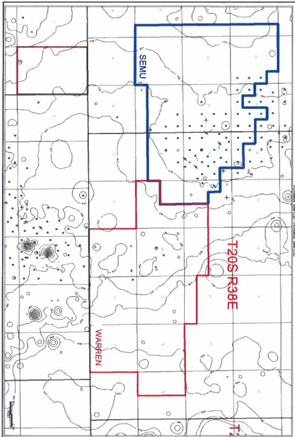
Top San Andres Structure Map
