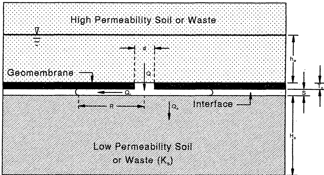
Figure 9. Leakage with Interfacial Flow Below Flawed Geomembrane
