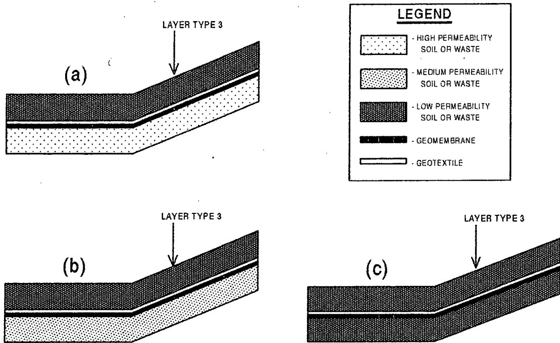
Figure 16. Geomembrane Liner Design Case 6
