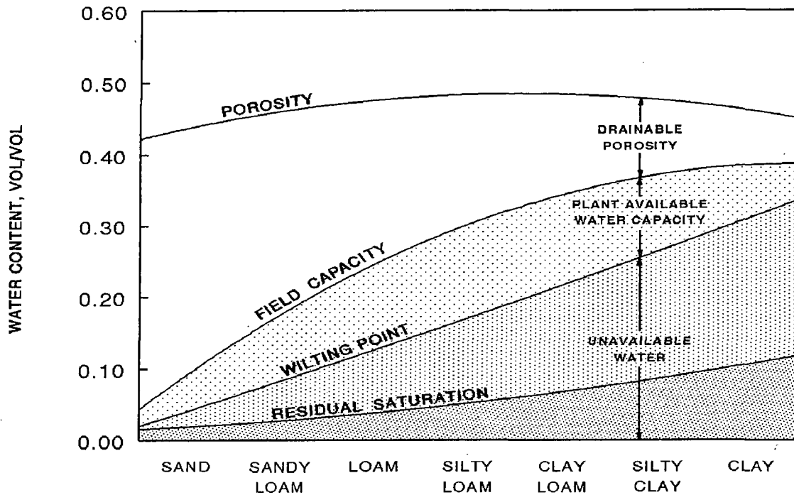
Figure 2. Relation Among Moisture Retention Parameters and Soil Texture Class
