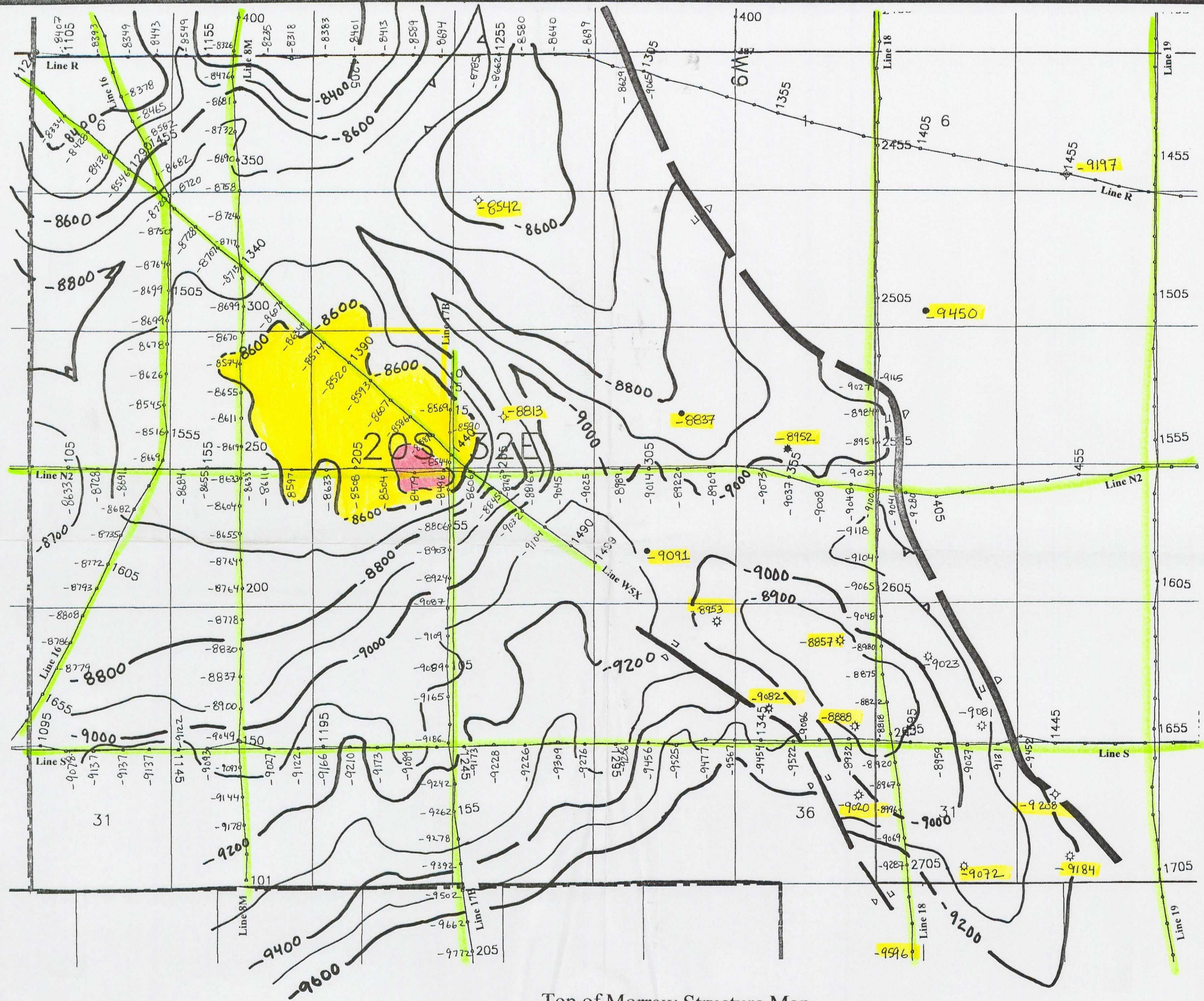
Top of Morrow Structure Map
