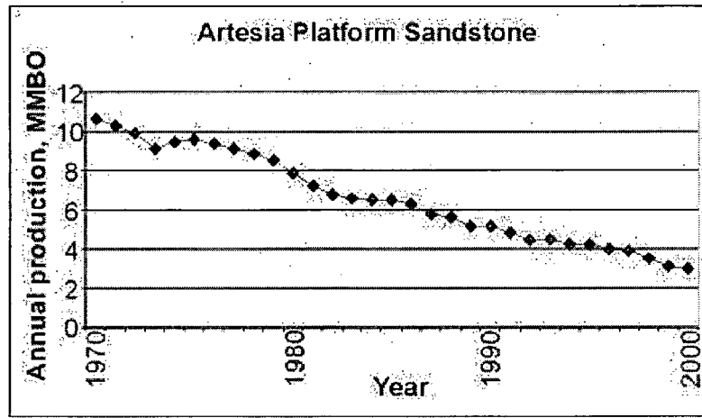
Figure 132-2. Historical annual production in southeast New Mexico from 1970 to 2000 from reservoirs with more than 1 MMBO cumulative production in the Artesia Platform sandstone play.
