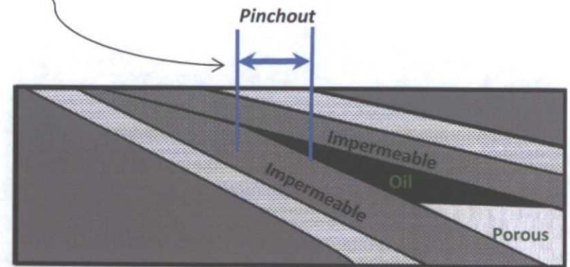
Depositional Model Schematic
