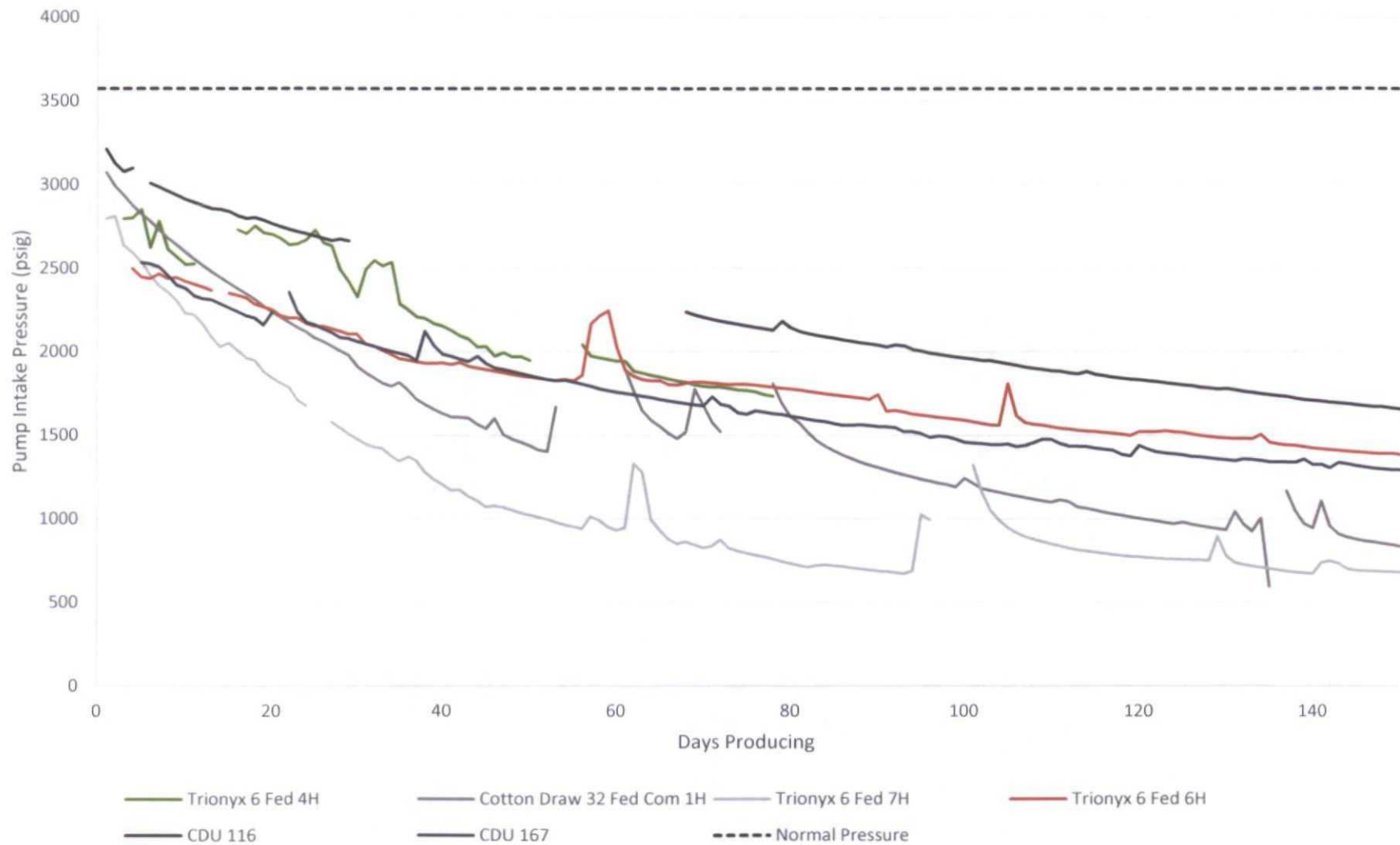
Pump Intake Pressure vs Producing Days
