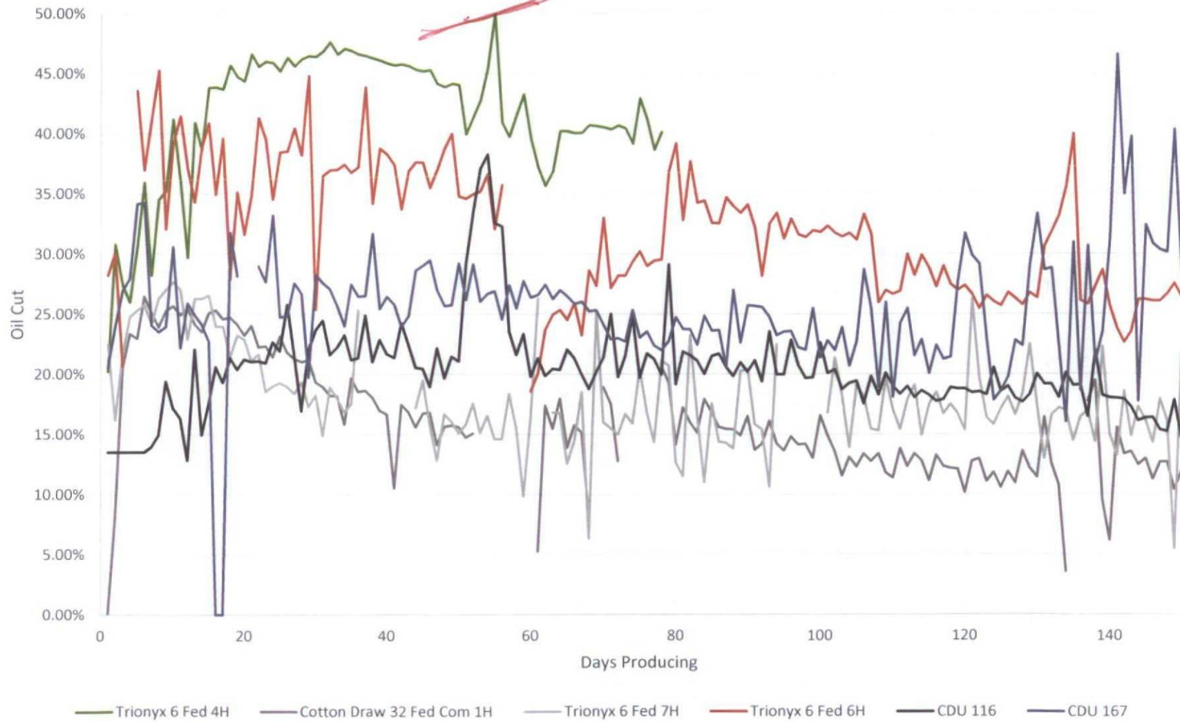
Oil Cut vs Producing Days
