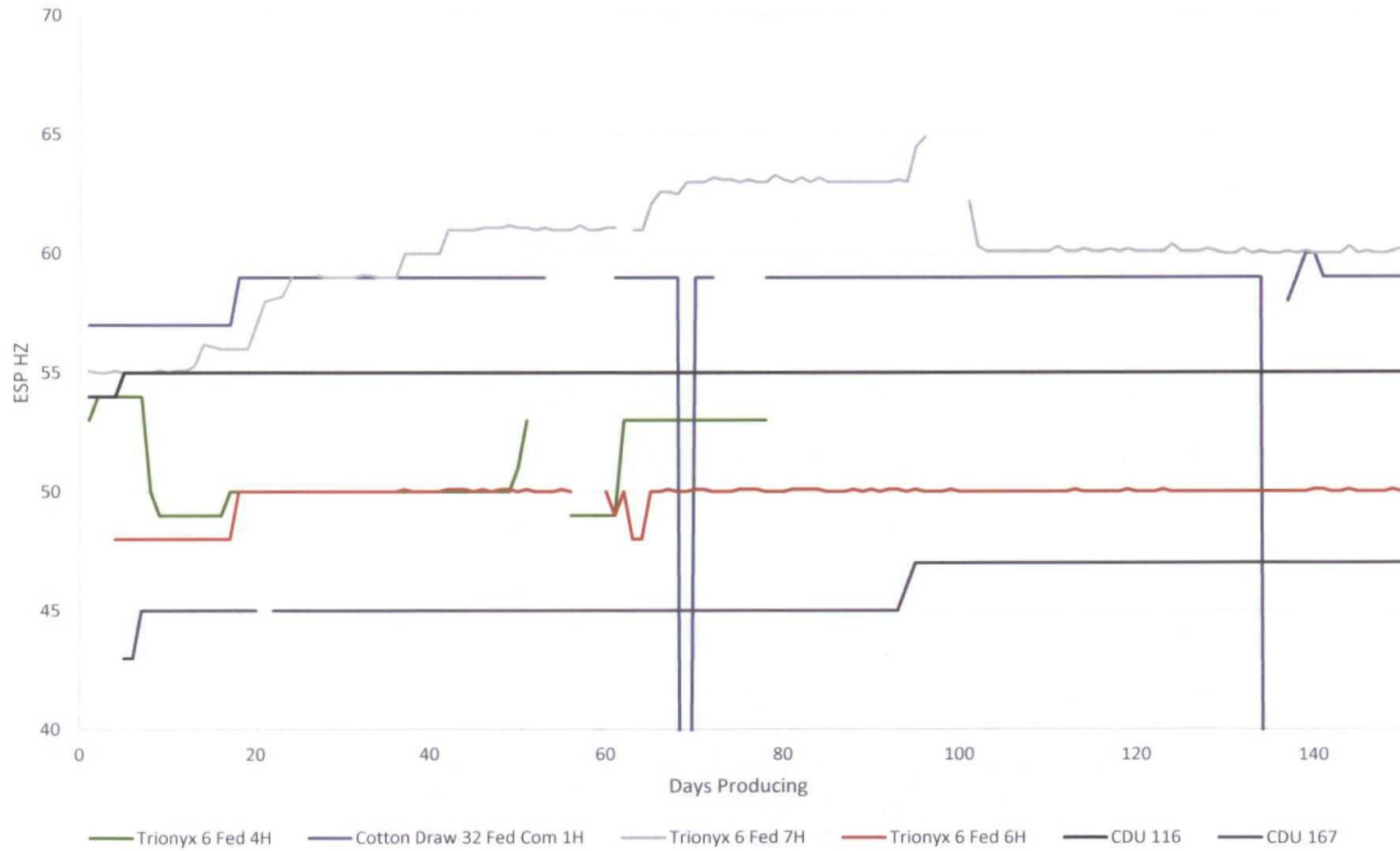
ESP HZ vs Producing Days
