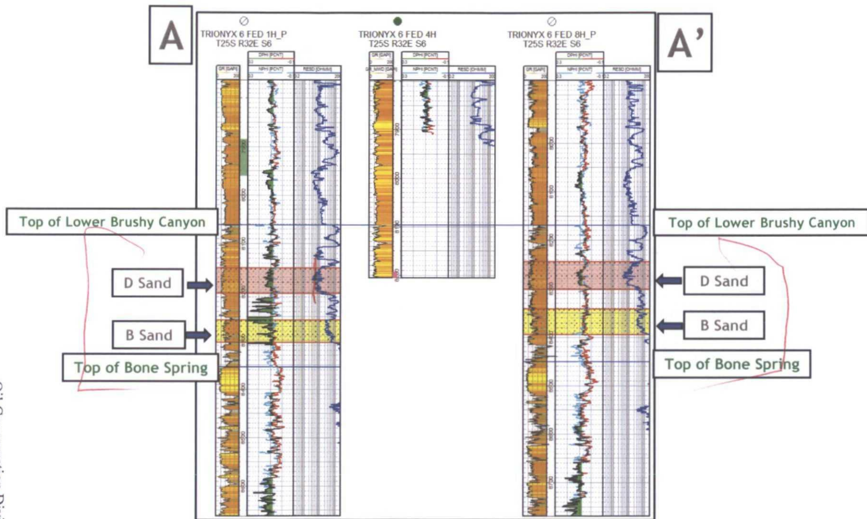
Cross Section A-A' Lower Brusy Canyon "B" and "D" Sandstones Geologist: Stephen Burns September 16, 2014
