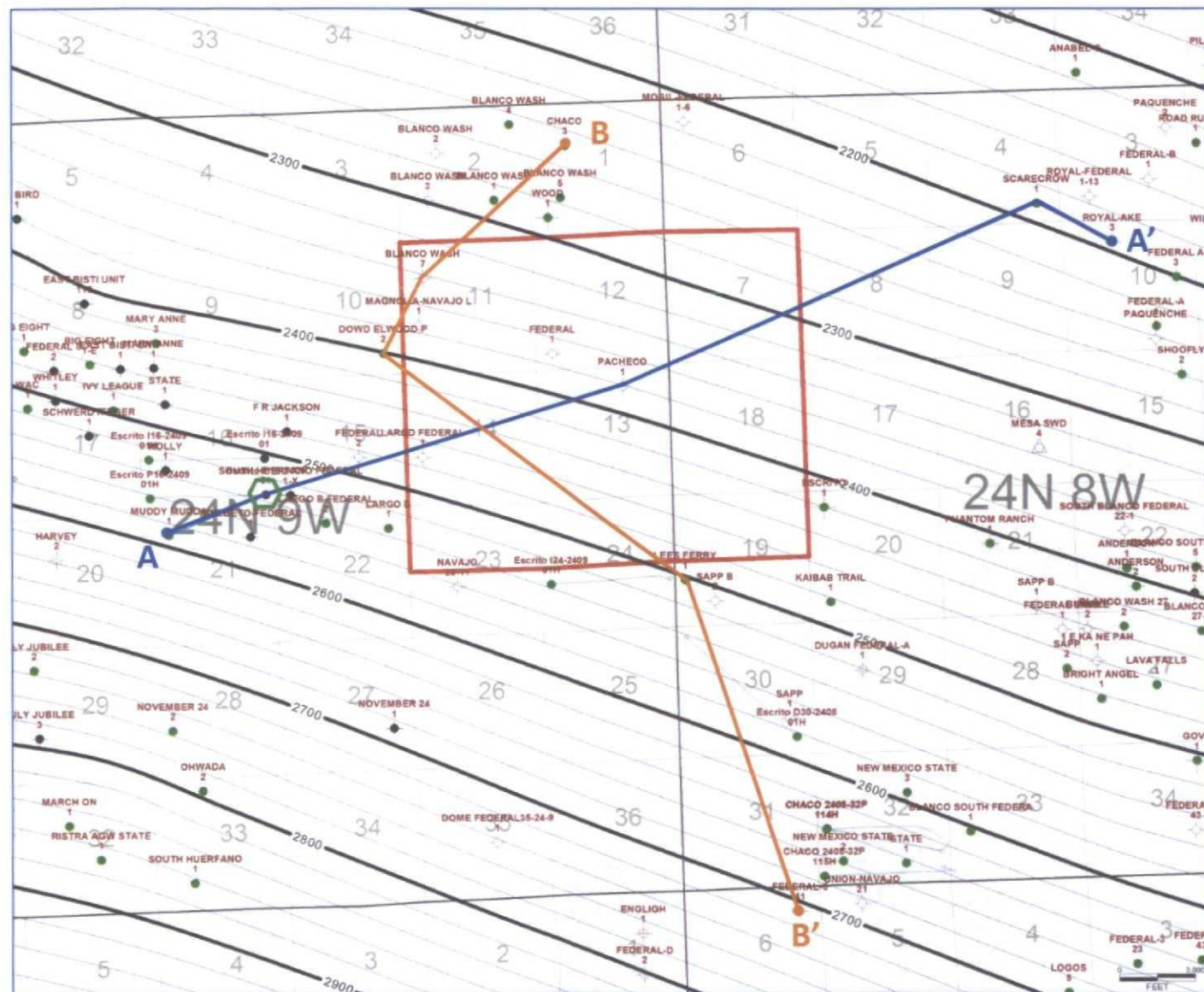
Top Mancos Structure Contour Map Sub-Sea True-Vertical Depth
