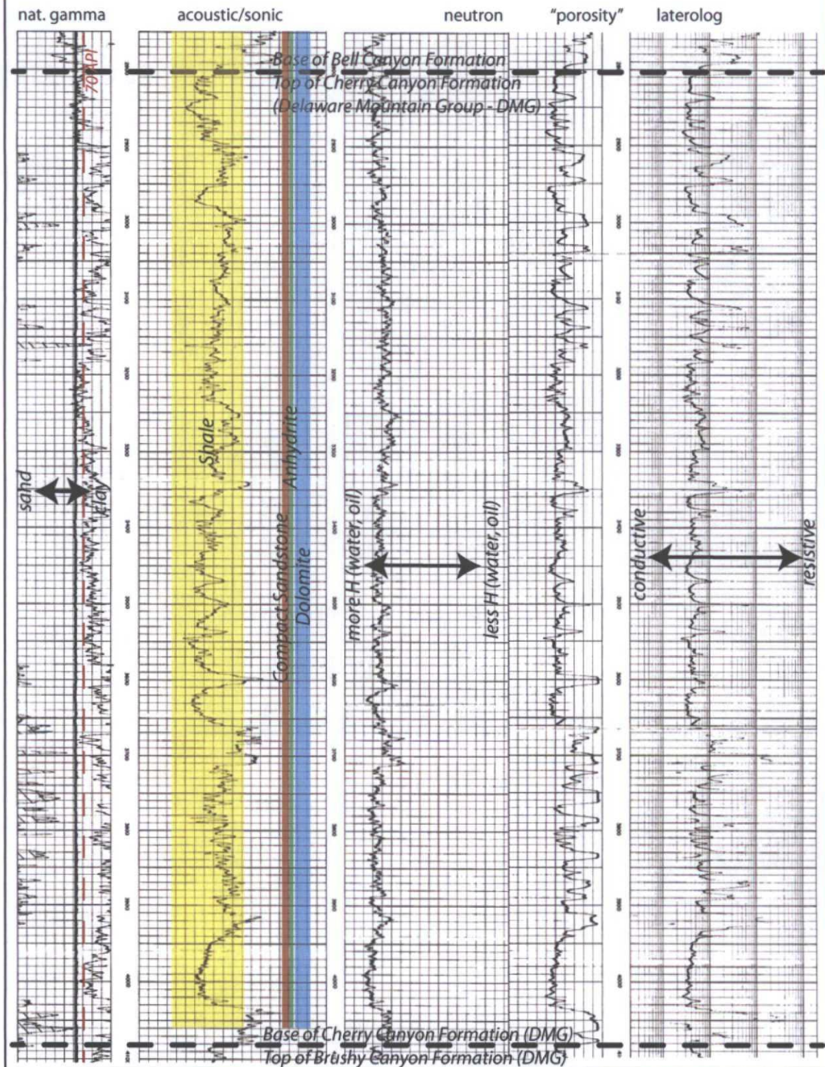
Figure 2 Log for Cherry Canyon Formation in Section 35, T22S, R26E, Airport Grace #1 (API 30-015-20829)
