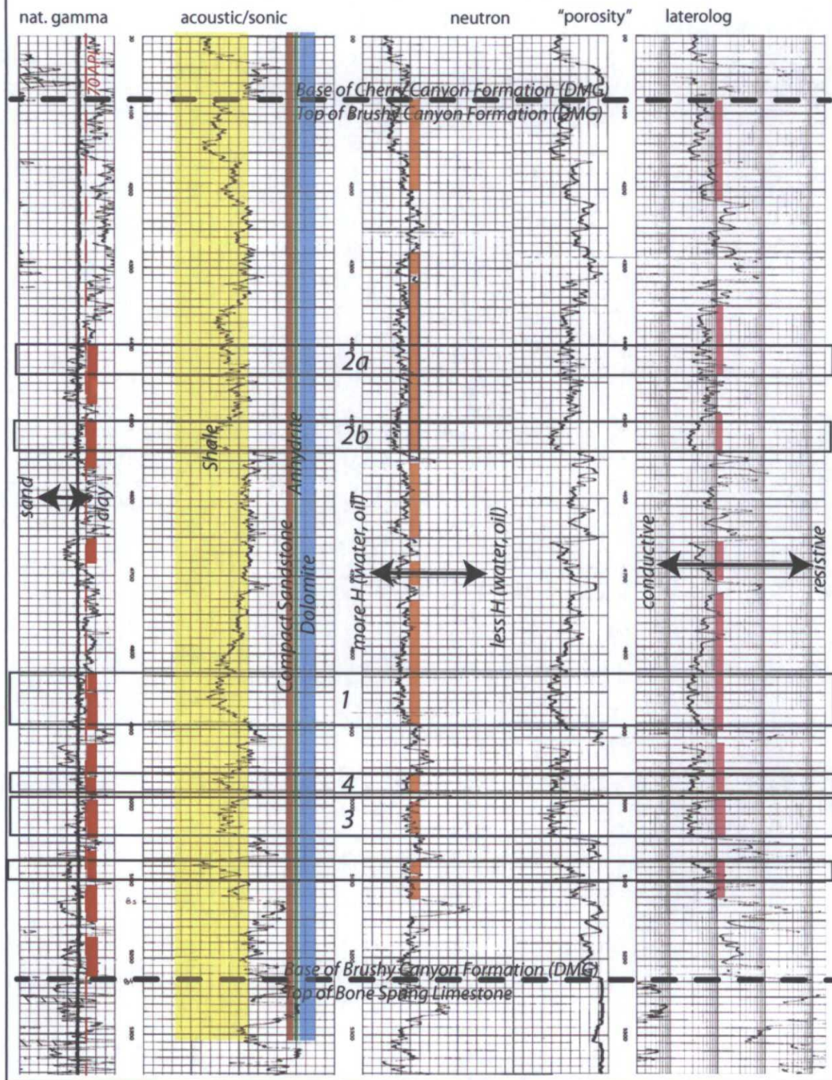
Figure 3 Log for Brushy Canyon Formation in Section 35, T22S, R26E, Airport Grace #1 (API 30-015-20829)
