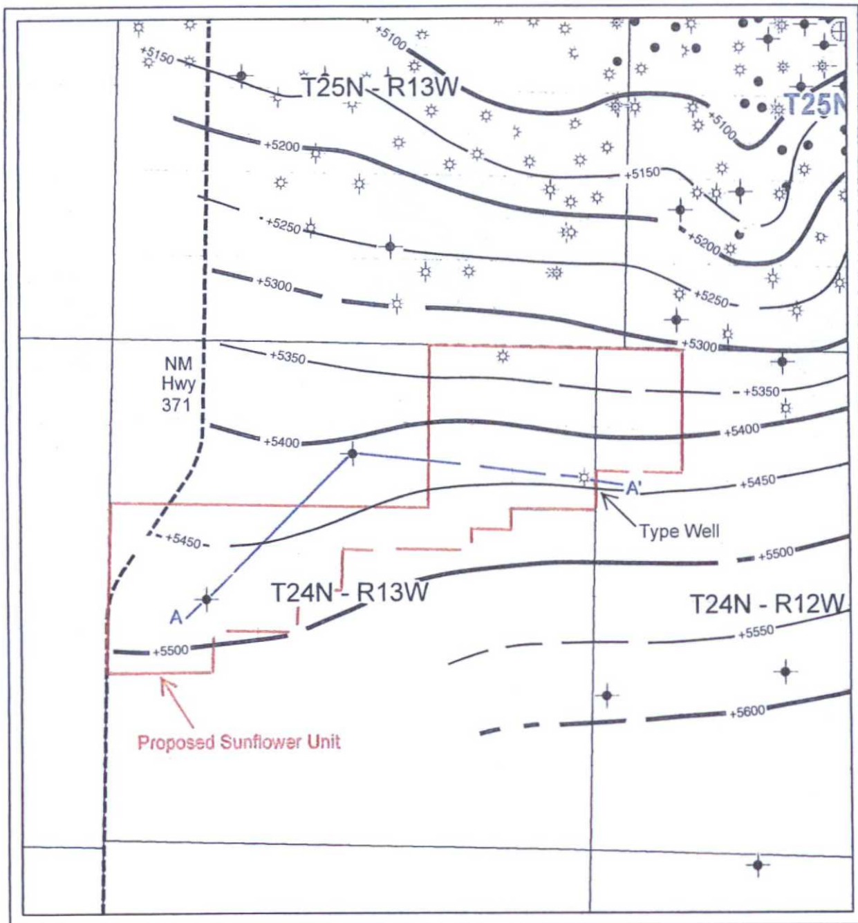
Figure 2. Structure contour map drawn on the top of the Pictured Cliffs Sandstone, showing the location of the proposed Sunflower Unit outline, type log and cross-section A-A' of wells shown in Figure 3 and Table 1. Contour Interval = 50-feet.
