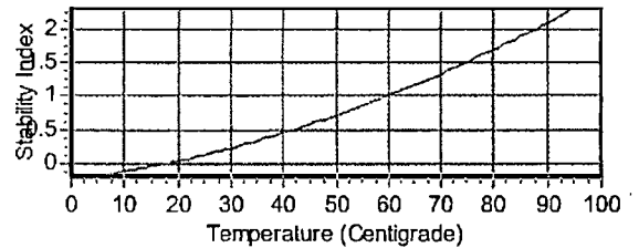
Calcium Sulfate Solubility
