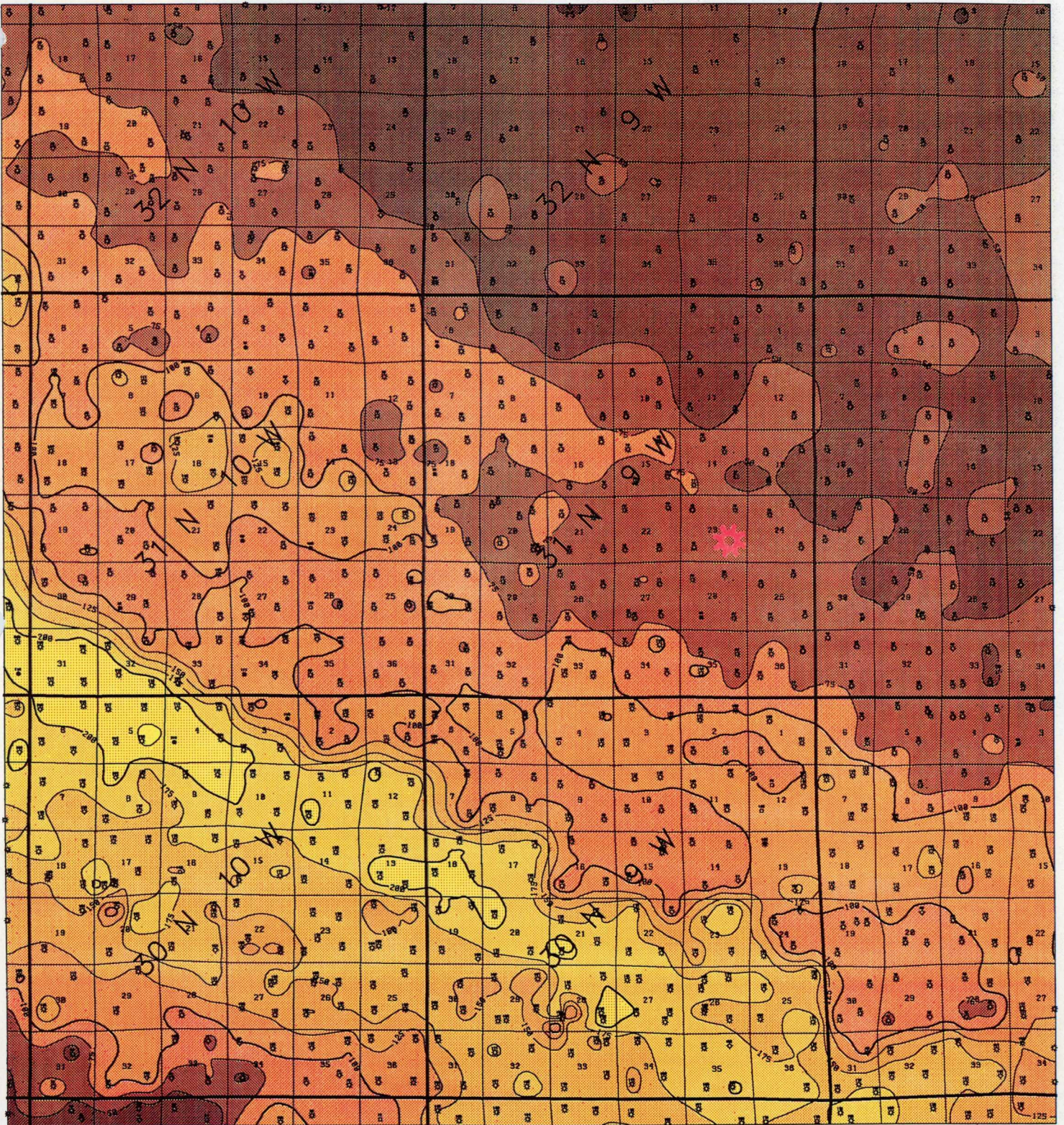
MERIDIAN OIL INC. SEYMOUR #7A (SE SEC 23, T31N - R9W) CONTOURED ISOPACH OF CLIFFHOUSE FORMATION CI = 25' Drawn B THIBODEUX Date 9-JAN-88 Checked
