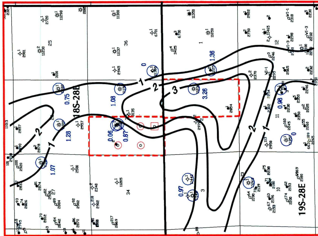
Isopach Map LOWER MORROW SAND porosity \times H ( \phi \geq 3.5\% ) C.I. = 1'
