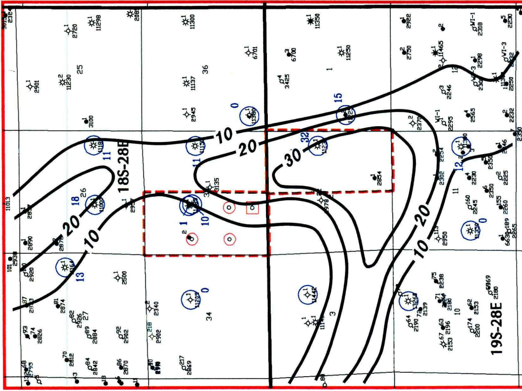
Isopach Map LOWER MORROW SAND H \geq 3.5\% porosity C.I. = 10'
