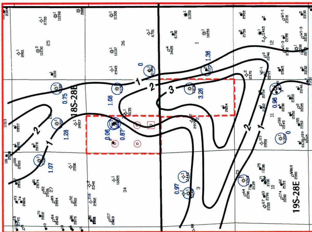
Isopach Map LOWER MORROW SAND porosity x H ( \phi \geq 3.5\% ) C.I. = 1'
