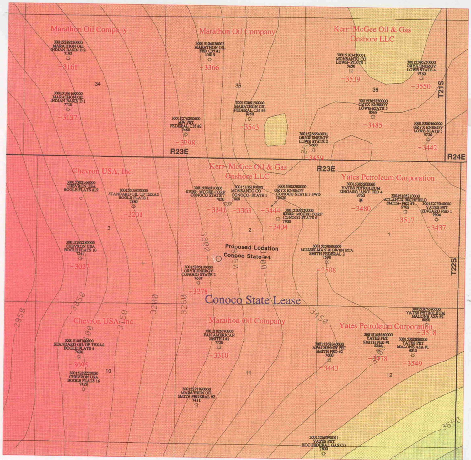
Structure Map: Top of Cisco Formation contours in feet below sealevel
