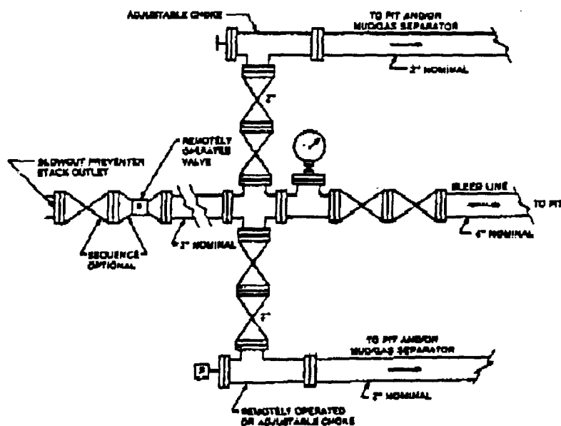
FIGURE K6-2. Typical choke manifold assembly for 5M rated working pressure service — surface installation.
