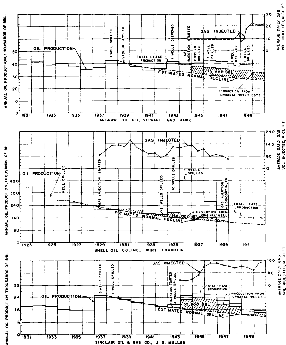
Figure 34. - Histories of gas injection on three successful projects, Healdton oil field, Carter County, Okla.
