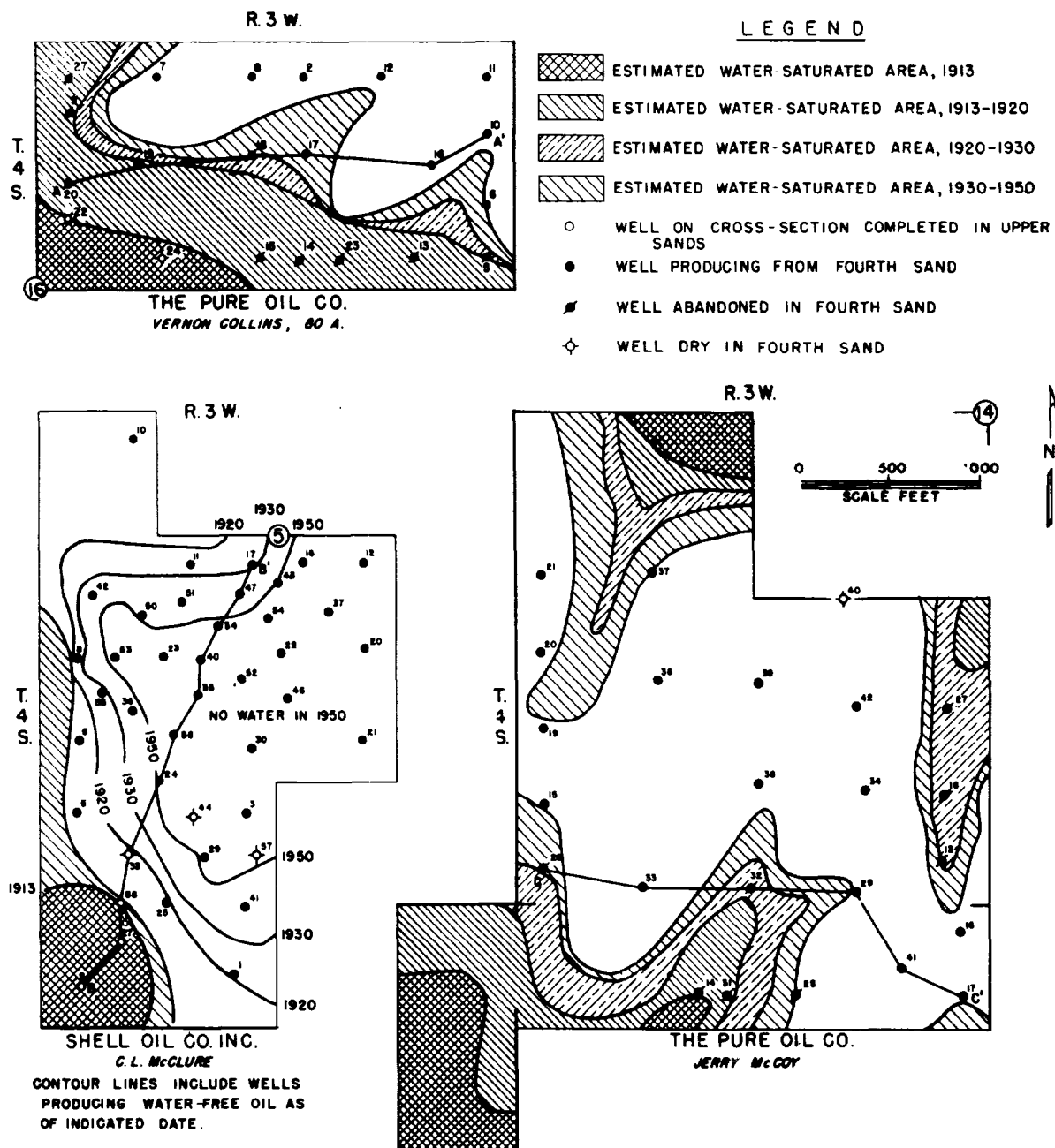
Figure 21. - Progressive advance of water in fourth Healdton sand underlying three leases, Healdton oil field, Carter County, Okla.
