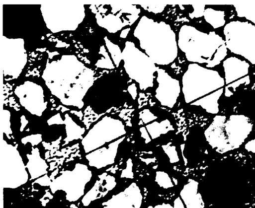
No. 41. Porosity 10.5 pct., Perm. 14 Md. Limestone 33.2 pct., Clay 4.5 pct.
