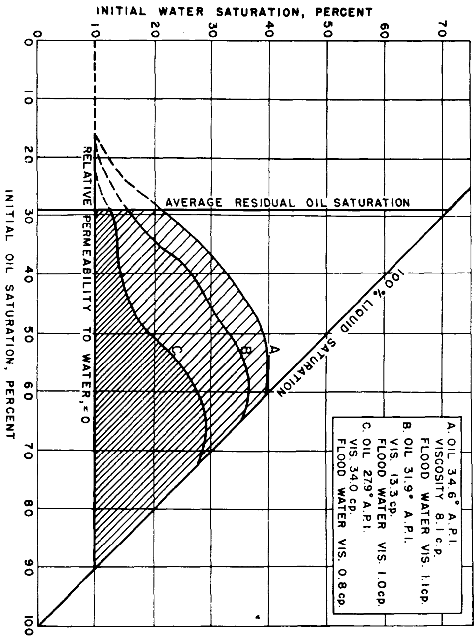
Figure 39. - Limiting initial liquid saturation for successful water flooding of loosely consolidated sands in the Healdton oil field.
