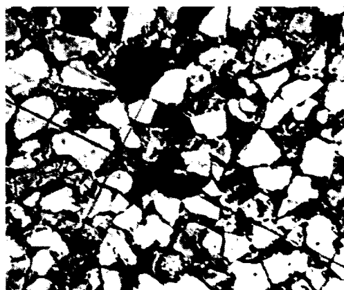
No. 40. Porosity 30.1 pct., Perm. 2900 Md. Limestone Trace, Clay 16.5 pct. Average grain size .255 mm.
