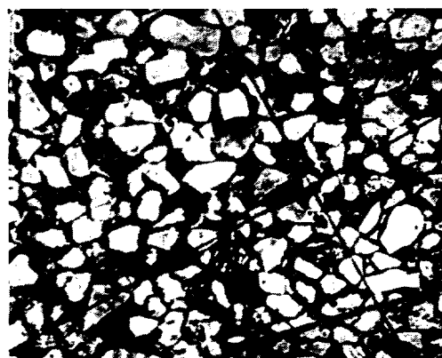
No. 31. Porosity 29.1 pct., Perm. 740 Md. Limestone 7.6 pct., Clay 2.2 pct. Average grain size .166 mm.
