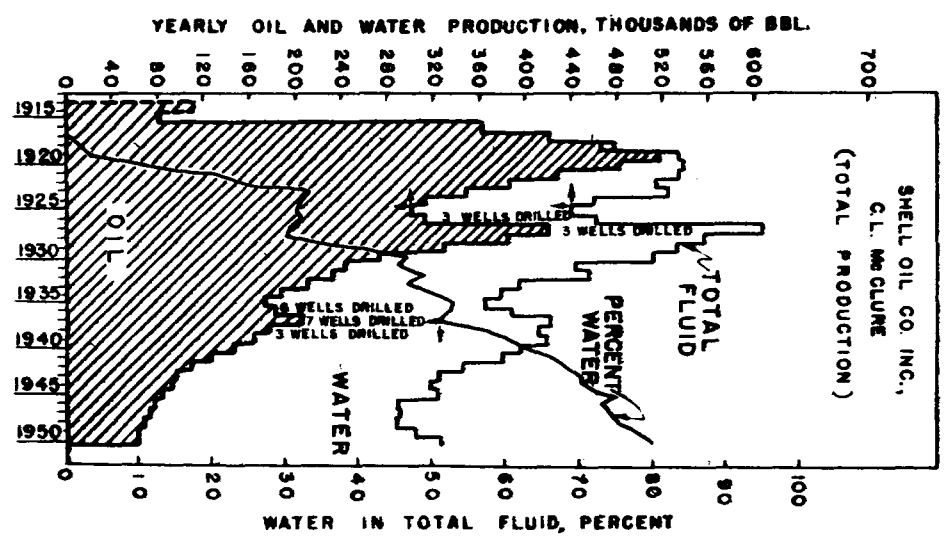
Figure 22. - Production histories of three leases with active water drive in fourth Healdton sand, Healdton oil field, Carter County, Okla.
