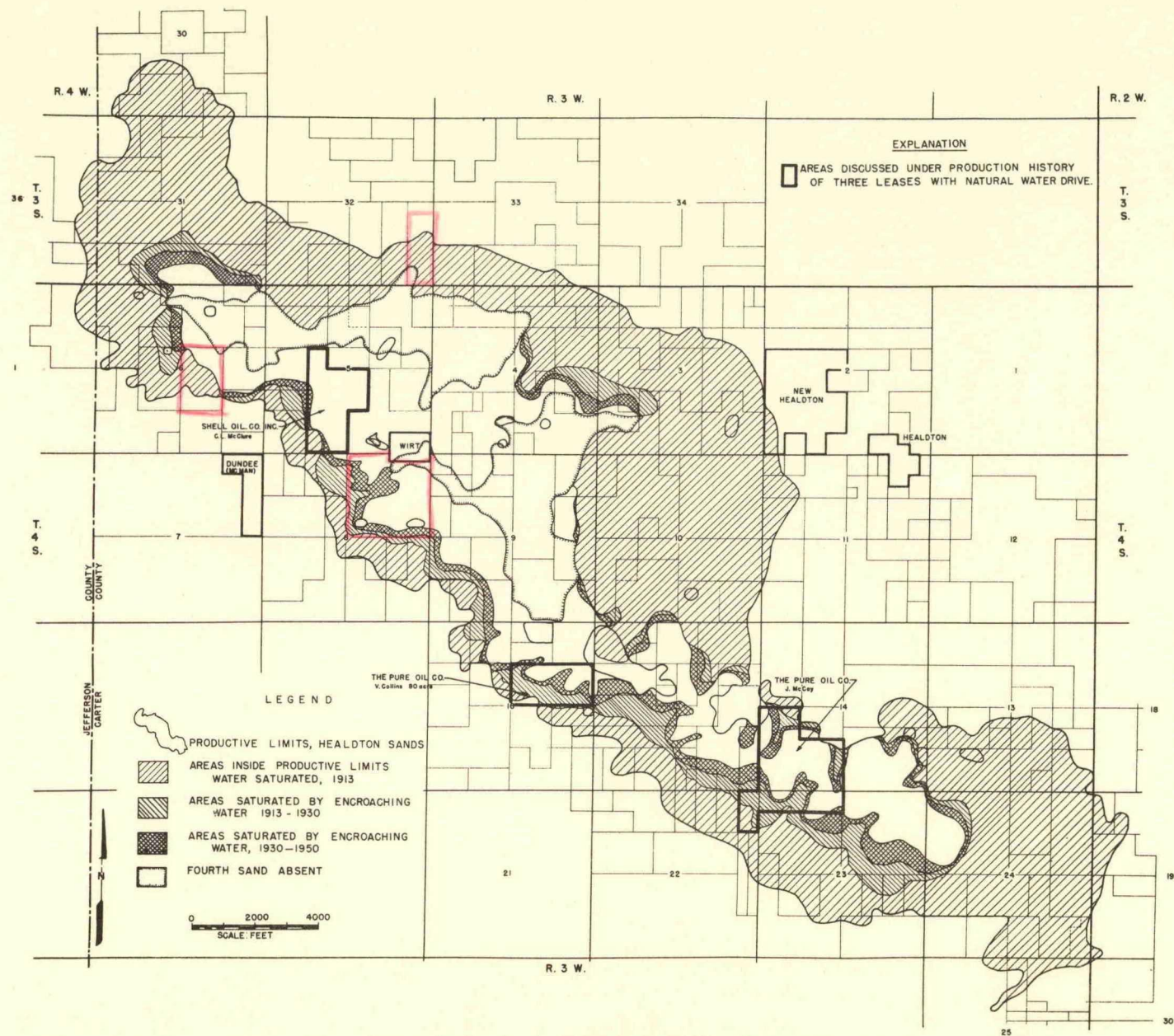
Figure 19. - Progressive advance of water in fourth Healdton sand, Healdton oil field, Carter County, Okla.
