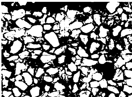
No. 12. Porosity 6.9 pct., Perm. 110 Md. Limestone 34.2 pct., Clay 5.5 pct. Average grain size .241 mm.
