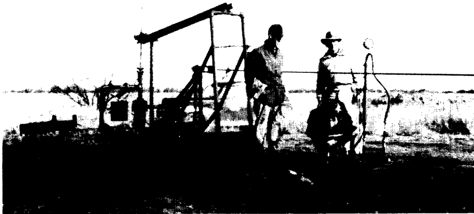
Figure 35. - Measuring produced gas from a well on a gas-injection lease, Healdton oil field, Carter County, Okla.
