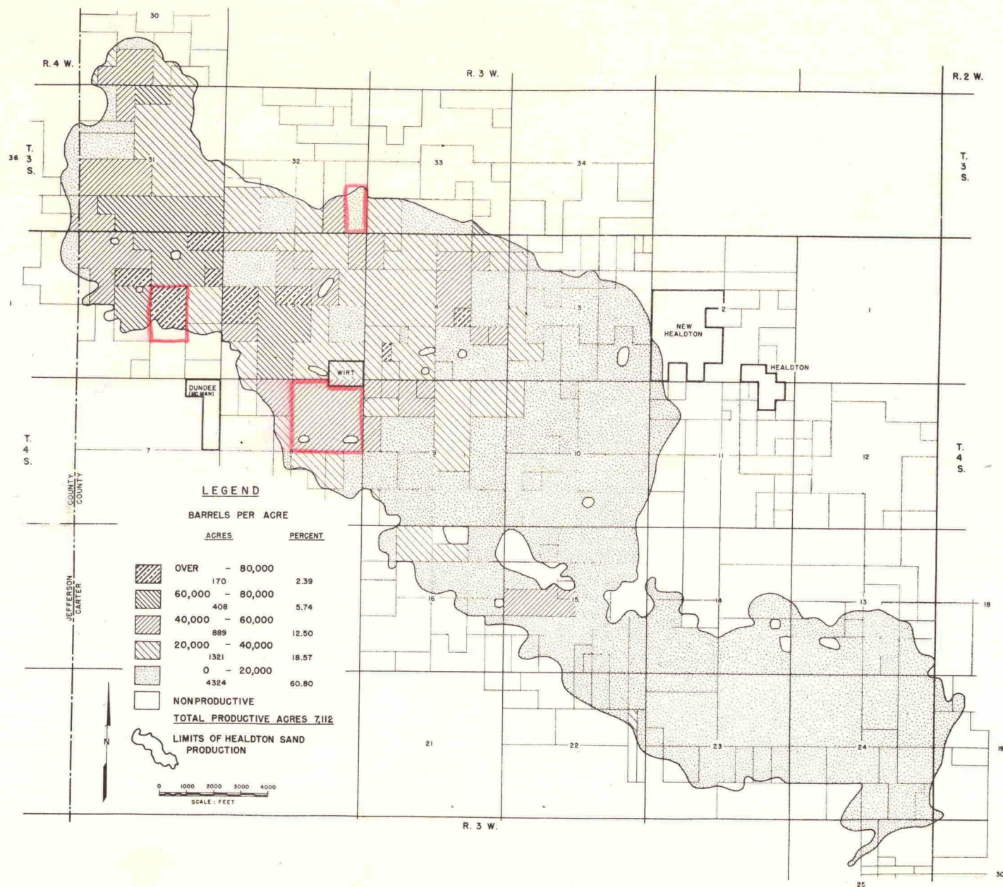
Figure 29. - Oil recovery from Healdton sands to January 1, 1935, Healdton oil field, Carter County, Okla.
