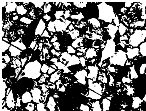
No. 7. Porosity 27.0 pct., Perm. 530 Md. Limestone 3.6 pct., Clay 13.4 pct. Average grain size .151 mm.
