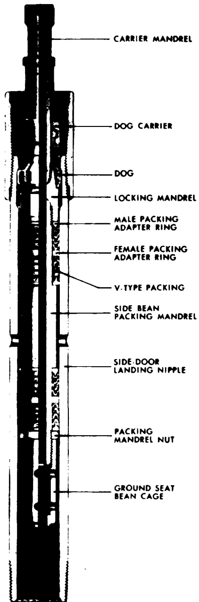
Otis Side-Door Choke and Landing Nipple
