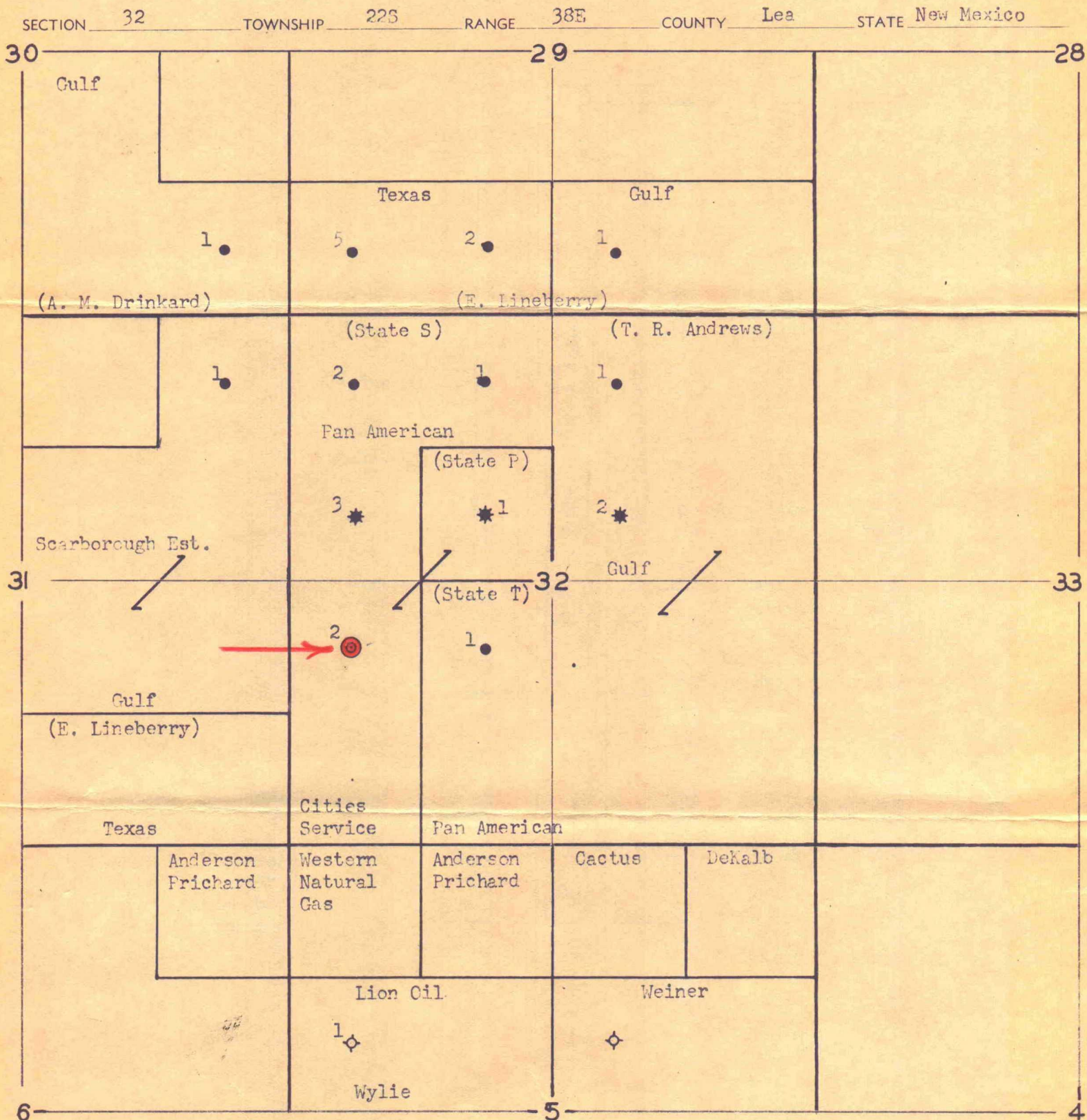
Plat showing location of Cities Service Oil Company's State "P" #2 Proposed Oil-Oil Dual Completion
