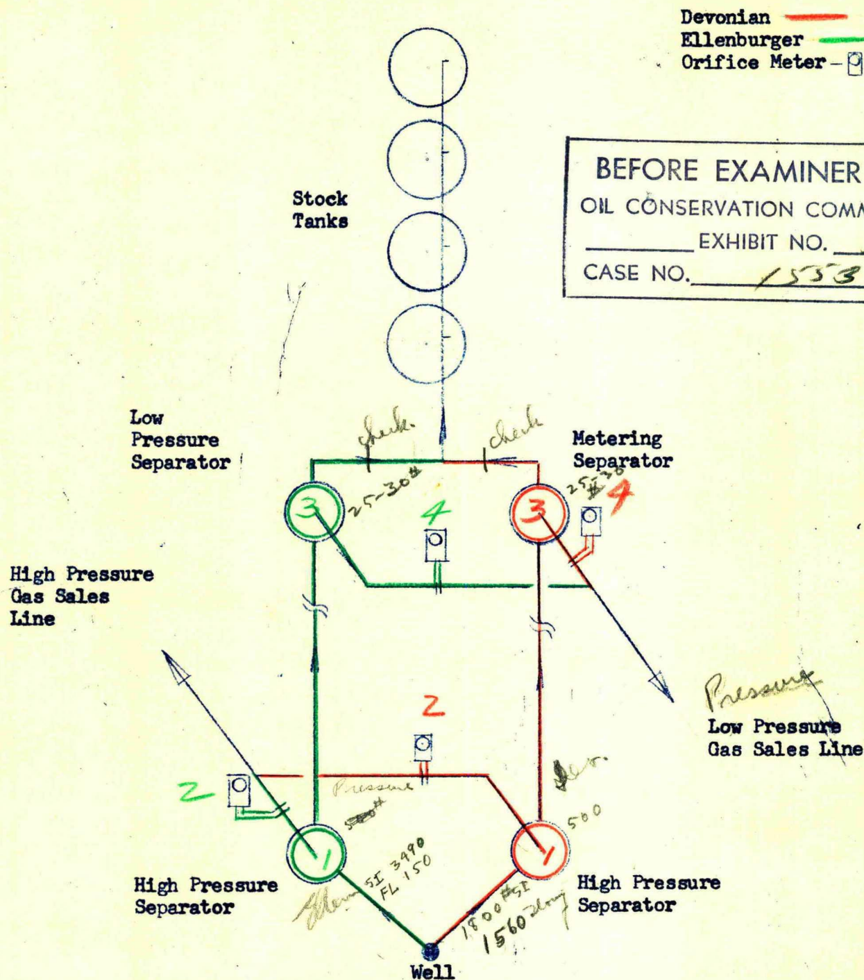
SCHEMATIC DIAGRAM OF PROPOSED HOOKUP FOR COMMINGLING, LIQUID AND GAS PRODUCTION
