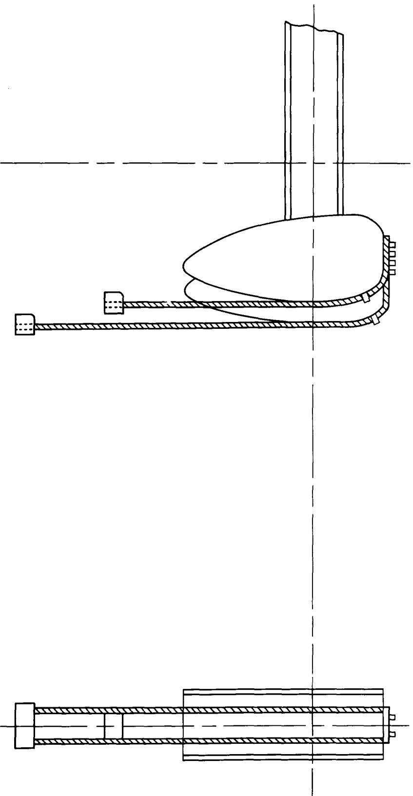
SIDE VIEW
