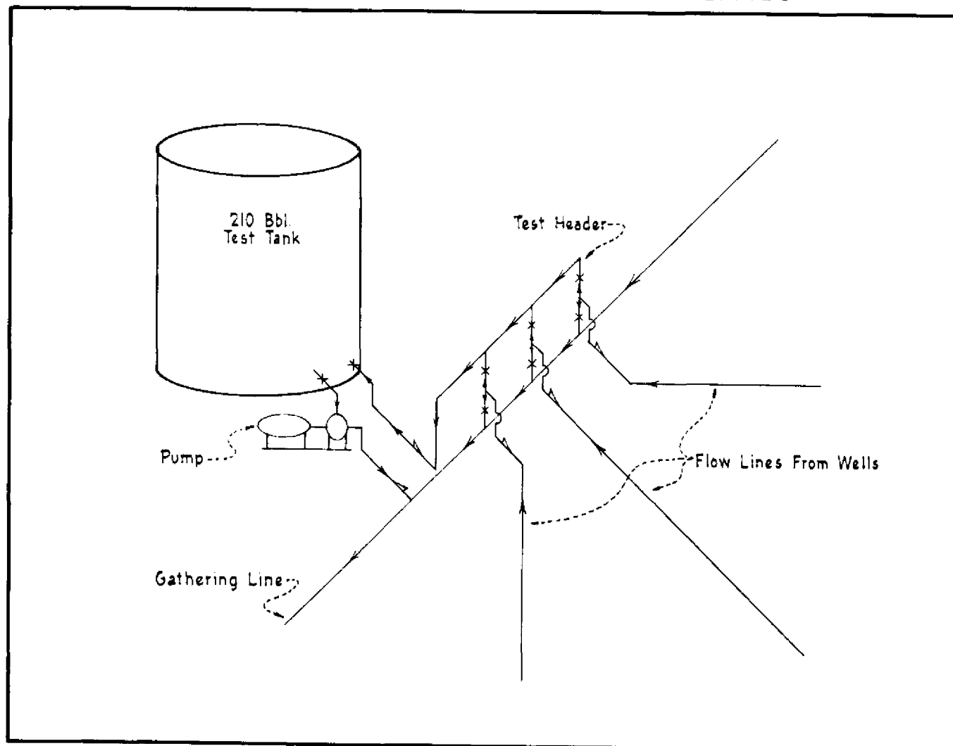
GREAT WESTERN DRILLING COMPANY PEBBLE UNIT SCHEMATIC DIAGRAM OF FLOW LINES, TANK BATTERY, AND TESTING FACILITIES
