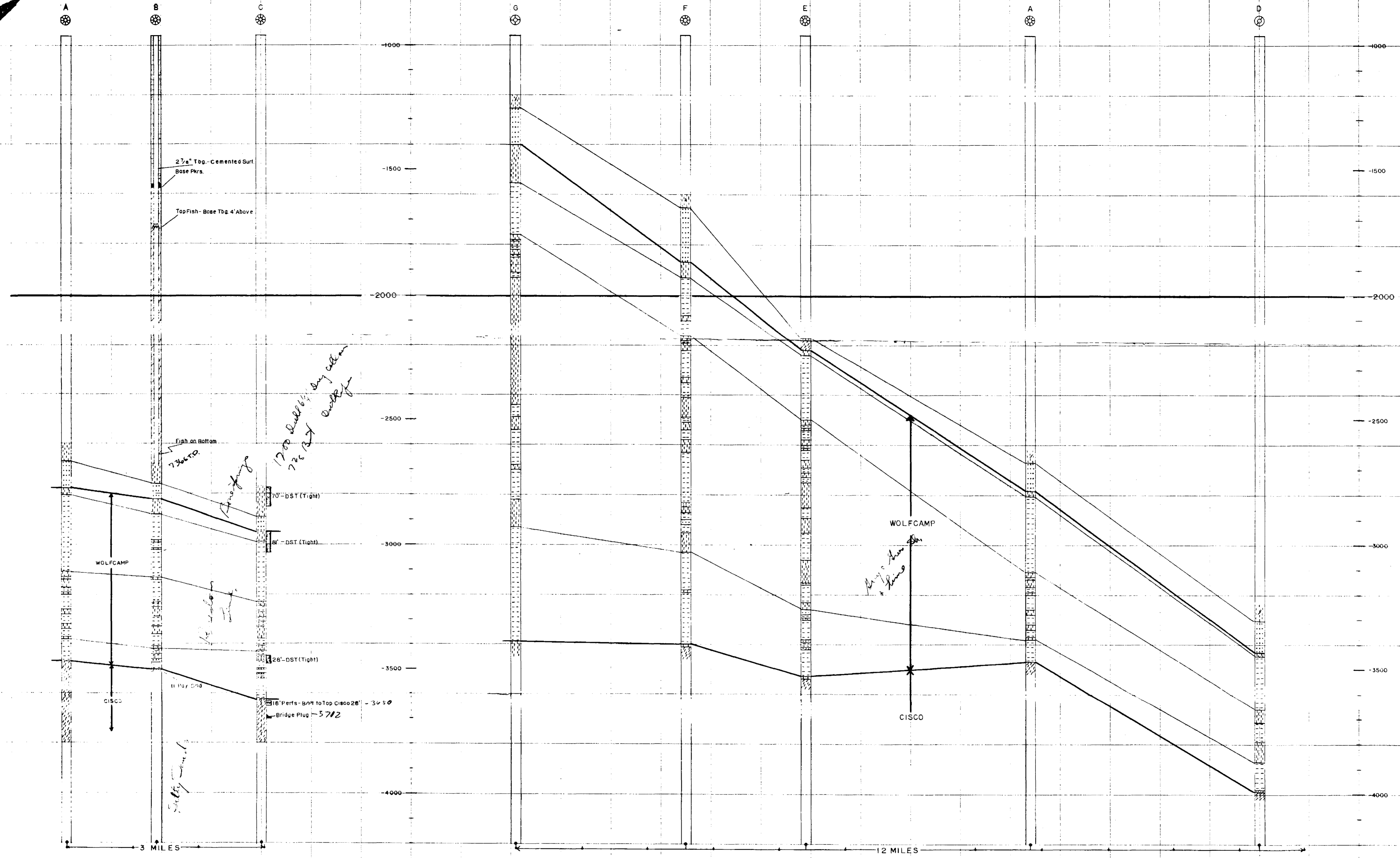
SW/NE SECTION — INDIAN HILLS FIELD — EDDY CO., N.MEX.
