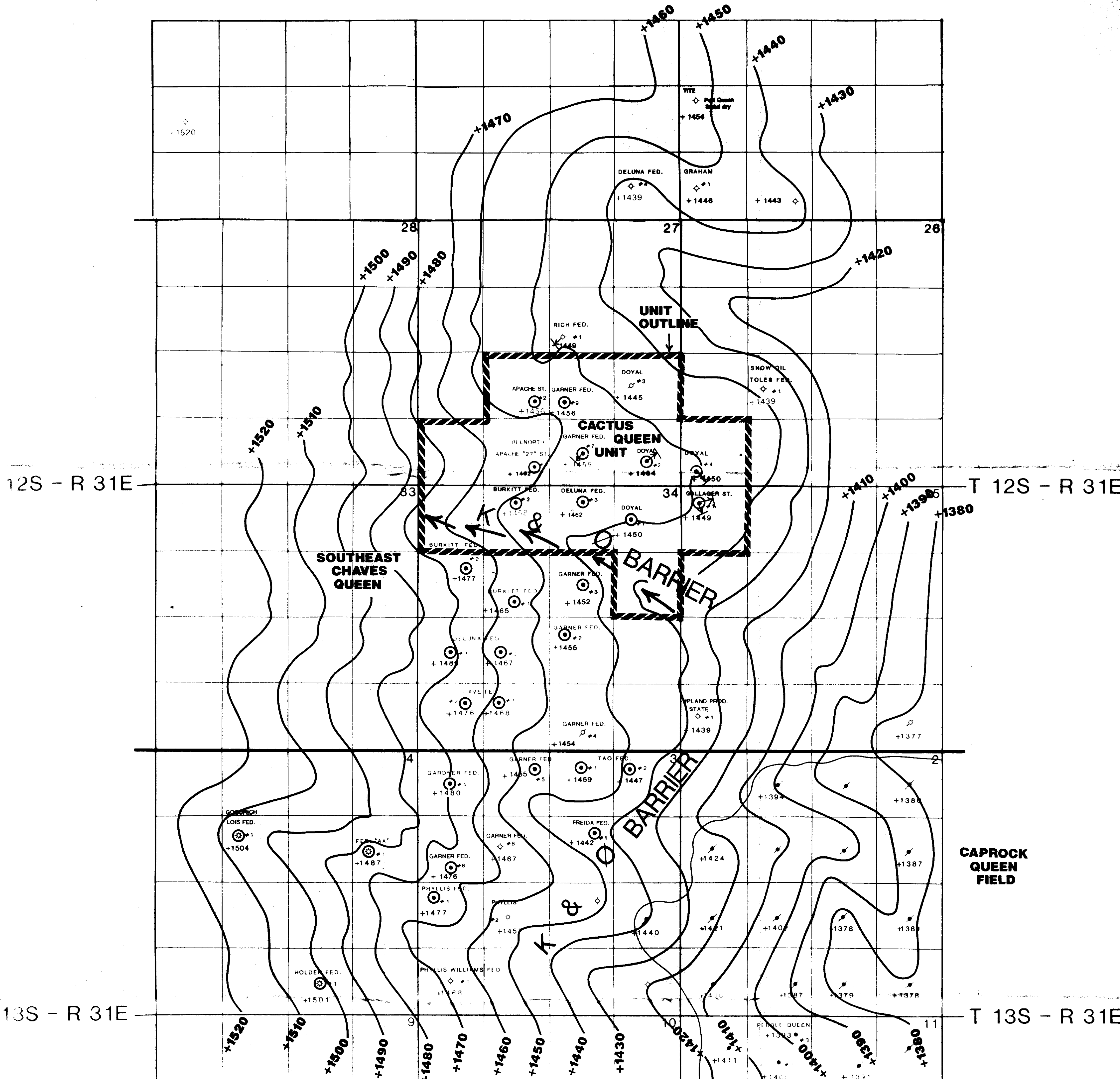
YATES DRILLING SE CHAVES QUEEN FIELD CHAVES CO., NM T 12 S - R 31 E QUEEN STRUCTURE ⊙ QUEEN PRODUCERS ○ ○ ○ OUTLINE CAPROCK QUEEN FIELD ← ← ← K & O BARRIER C.I. = 10' SCALE: 1" = 1000' FIGURE #3
