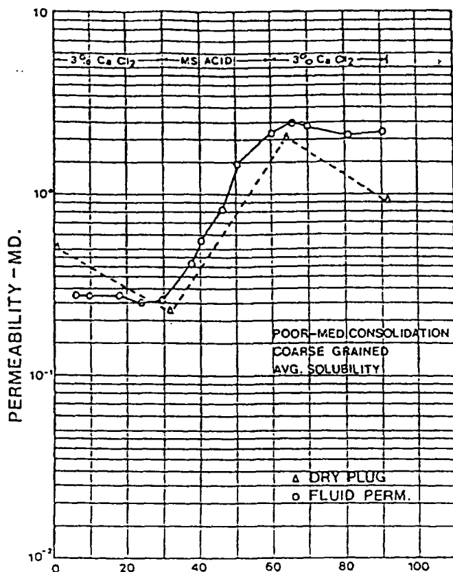
FIGURE 6 — CUMULATIVE EFFLUENT—ML.
