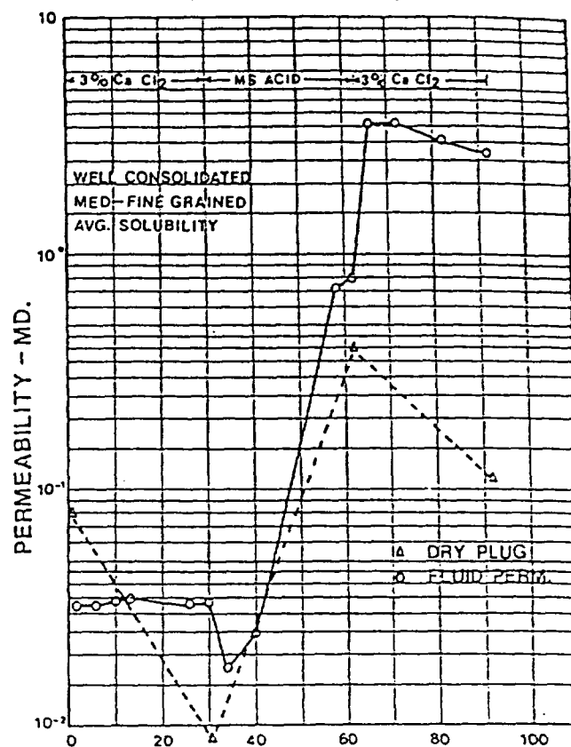
FIGURE 9 — CUMULATIVE EFFLUENT—ML.
