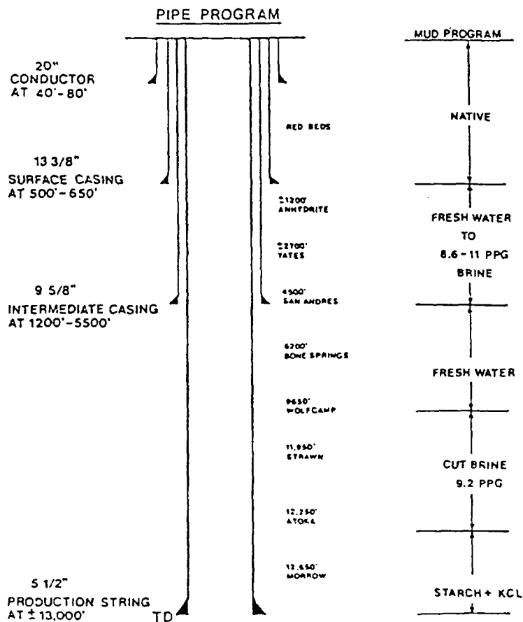
FIGURE 10 — TYPICAL MORROW CASING PROGRAM
